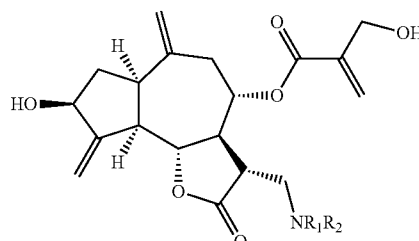
Aminocyanaropicrins
