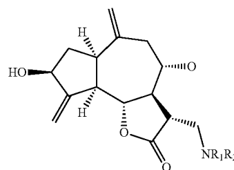
Aminodesacylcyanaropicrins
