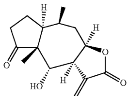
11,13-Dihydrohelenalin
