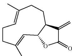
Costunolide
