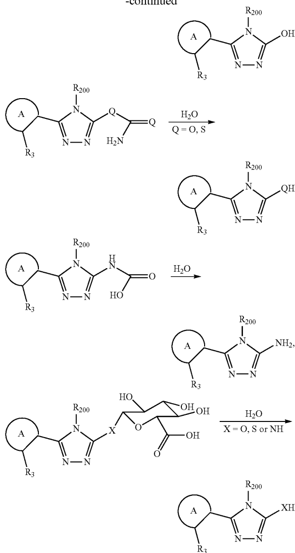
Scheme I: Synthesis of triazole compounds of the invention
