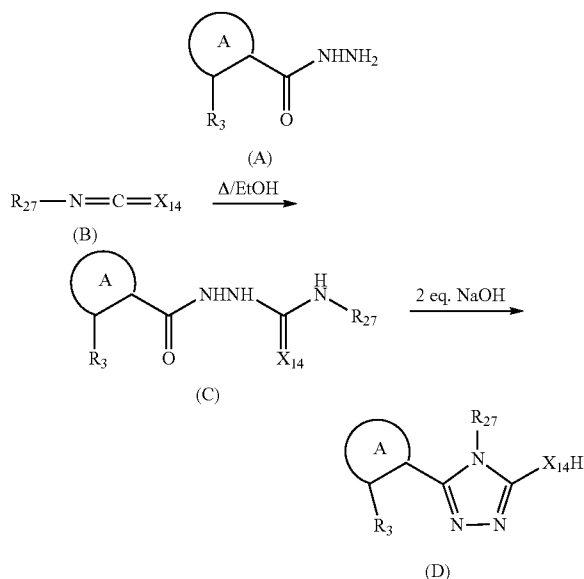
Scheme I: Synthesis of triazole compounds of the invention
