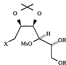
(10) X = OMs; R, R = \text{CMe}_2 (11) X = \text{N}_3 ; R, R = \text{CMe}_2 (12) X = \text{N}_3 ; R, R = H
