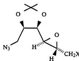
(14) X = \text{CH}_2\text{CO}_2^t\text{Bu} (15) X = CN
