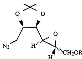
(6) R = H (7) R = TBDMS (8) R = TBDPS (9) R = \text{SO}_2\text{CF}_3
