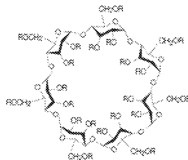
generic \beta -cyclodextrin
