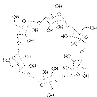
\gamma -cyclodextrin
