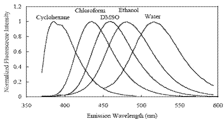
PRODAN Emission Spectra in Various Solvents
