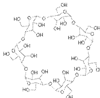
\beta -cyclodextrin
