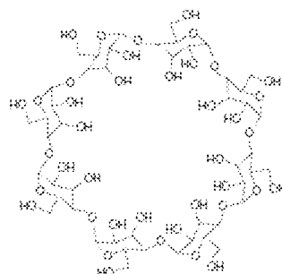
\gamma -cyclodextrin
