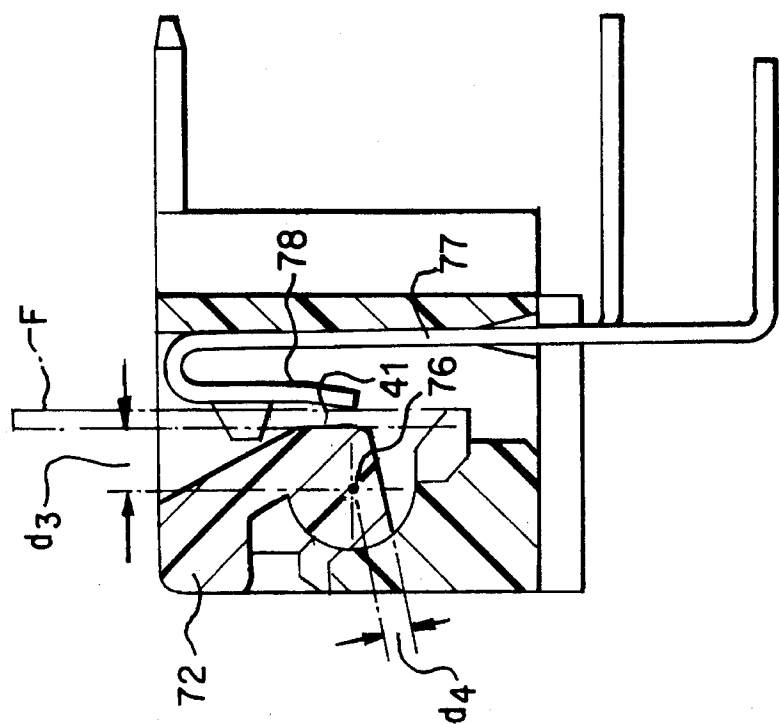
FIG. 7 PRIOR ART
