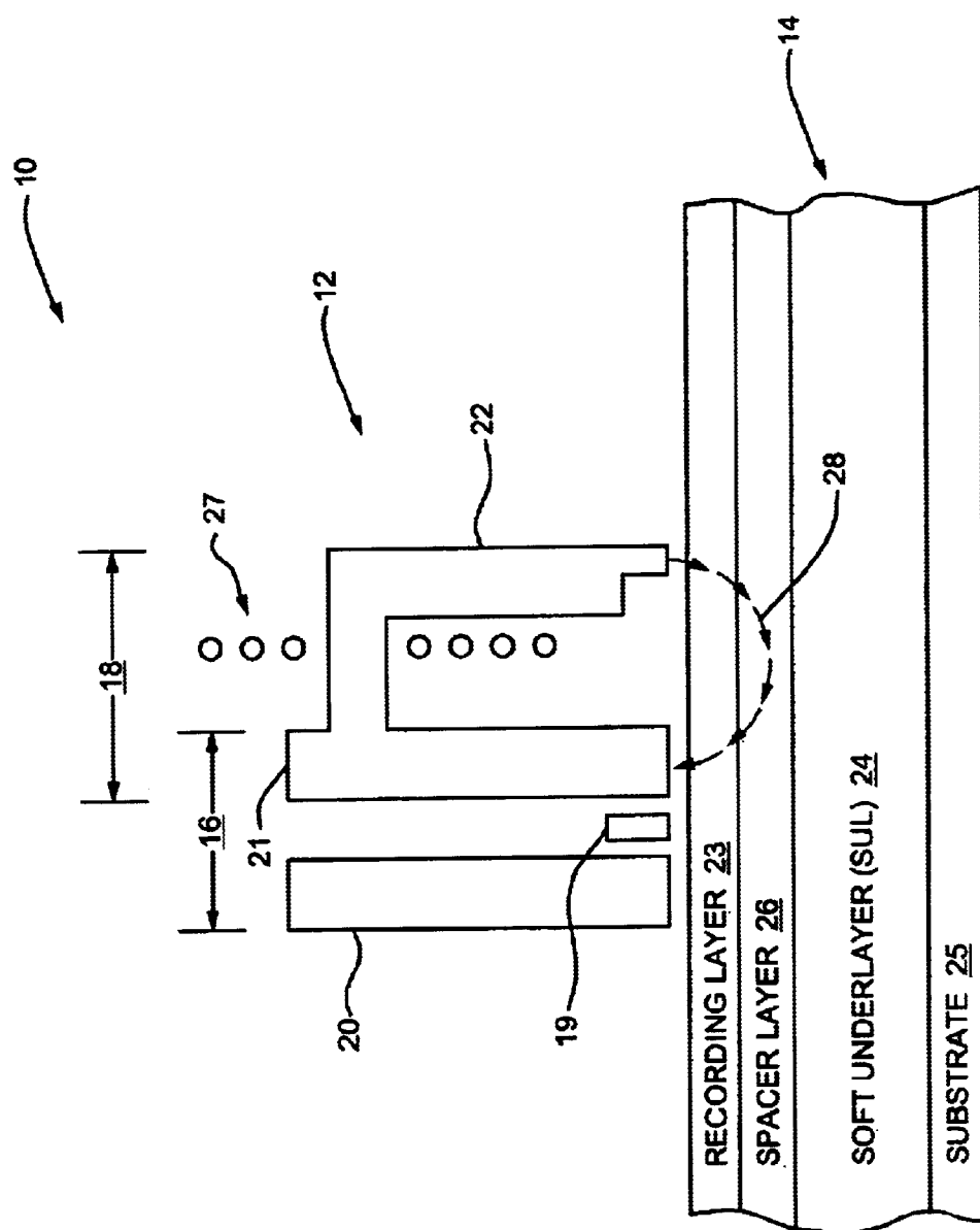
FIG. 1 (PRIOR ART)
