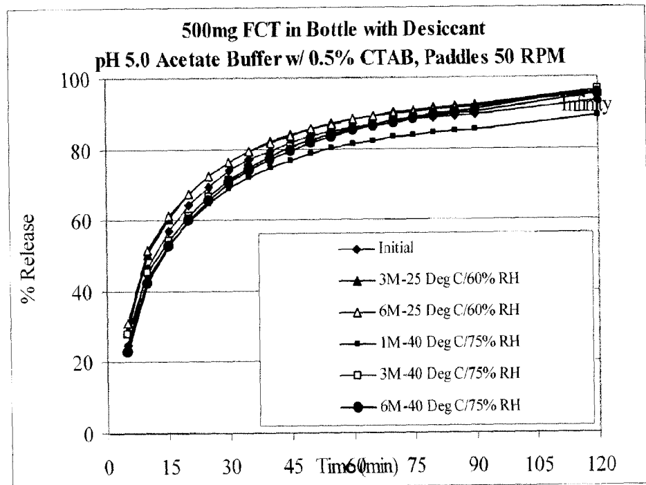
Figure 18: Dissolution of Croscarmellose based SKI-0606 formulation on accelerated stability in Bottles with Desiccant for 500 mg coated tablets
