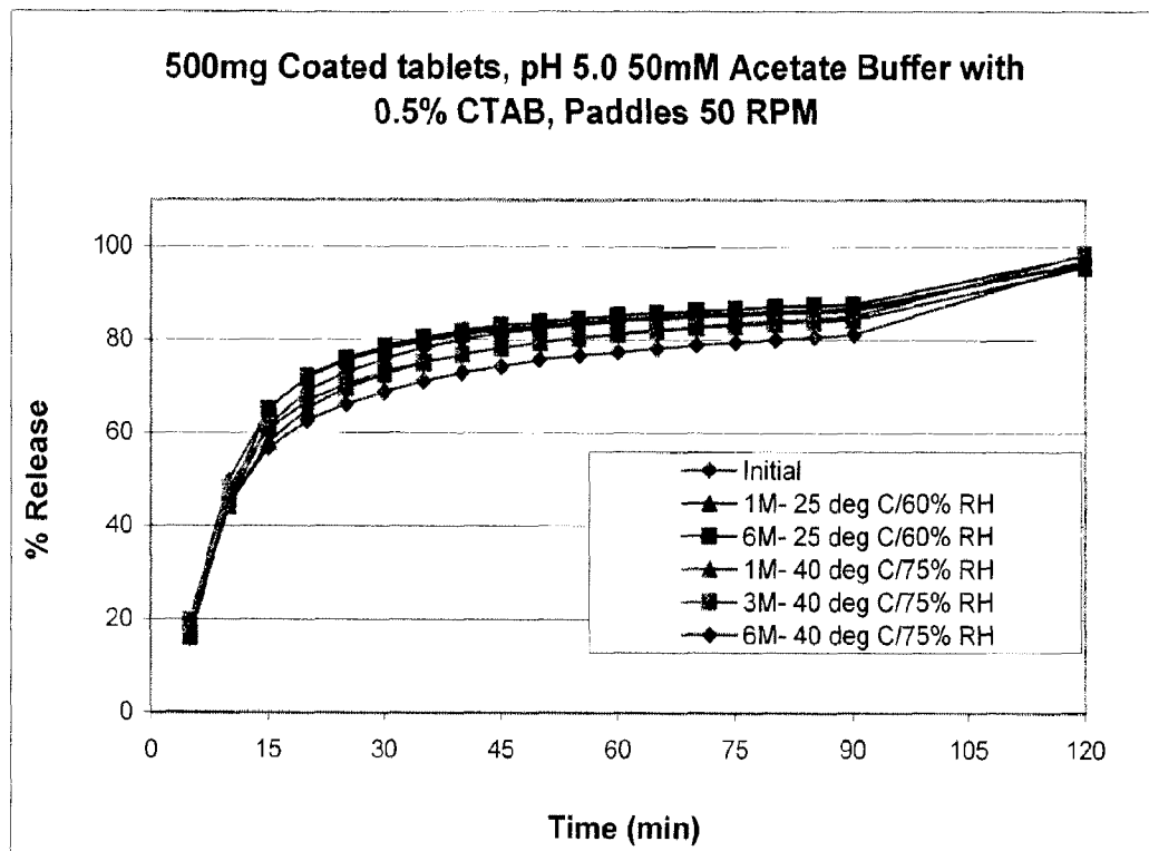
Figure 21: Scale-up (100 Kg) batch dissolution stability in Bottles with desiccant A
