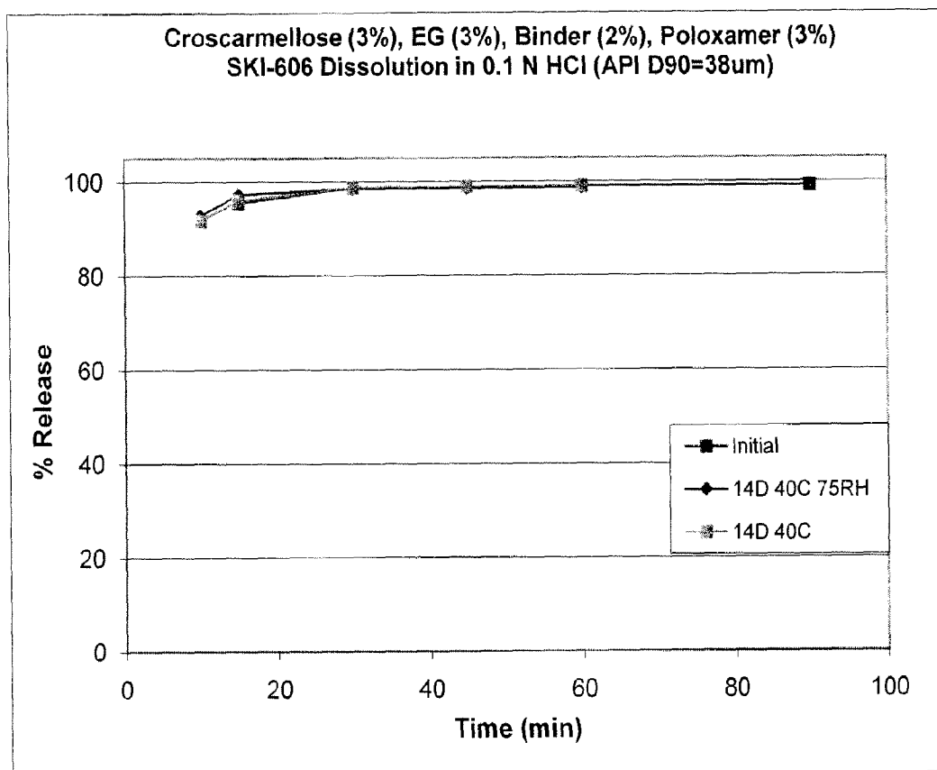
Figure 3. 14 day Dissolution on accelerated open dish stability in 0.1N HCl at 40°C and 40° C/75% RH for a model SKI-606 formulation containing Croscarmellose sodium.
