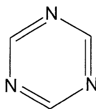
triazine
