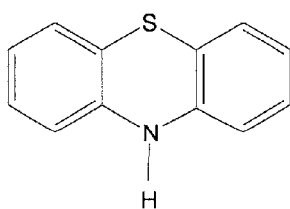
phenothiazine
