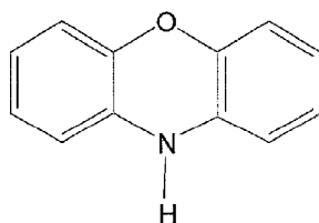
phenoxazine
