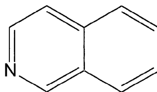
isoquinoline
