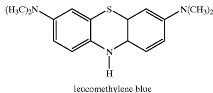
leucomethylene blue
