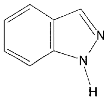
indazole
