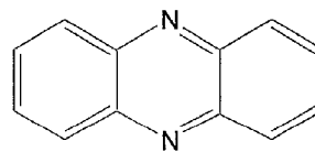
phenazine
