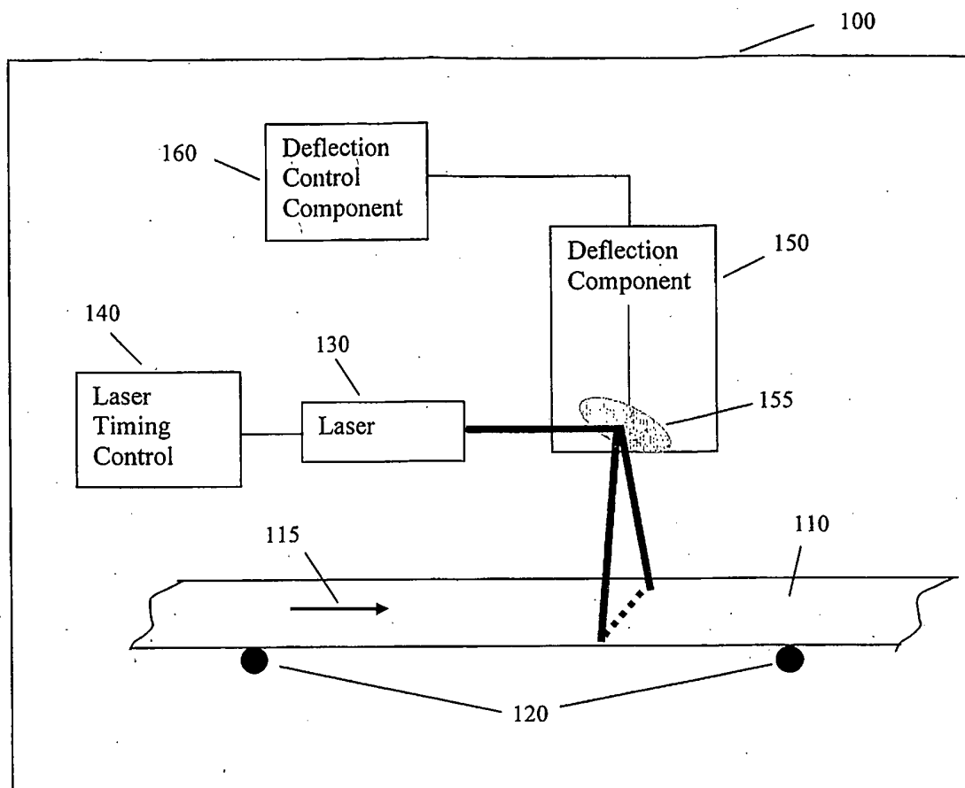
Fig 7. Block diagram of one embodiment of the across-track formatting system.
