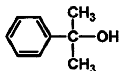
cumyl alcohol
