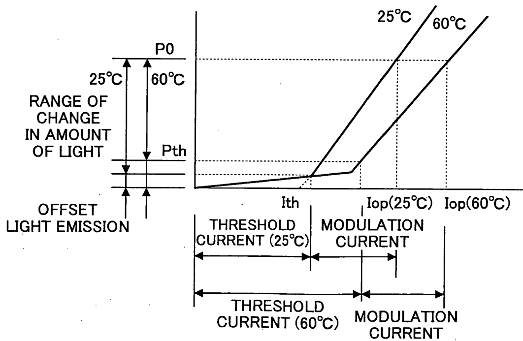
FIG.6 PRIOR ART
