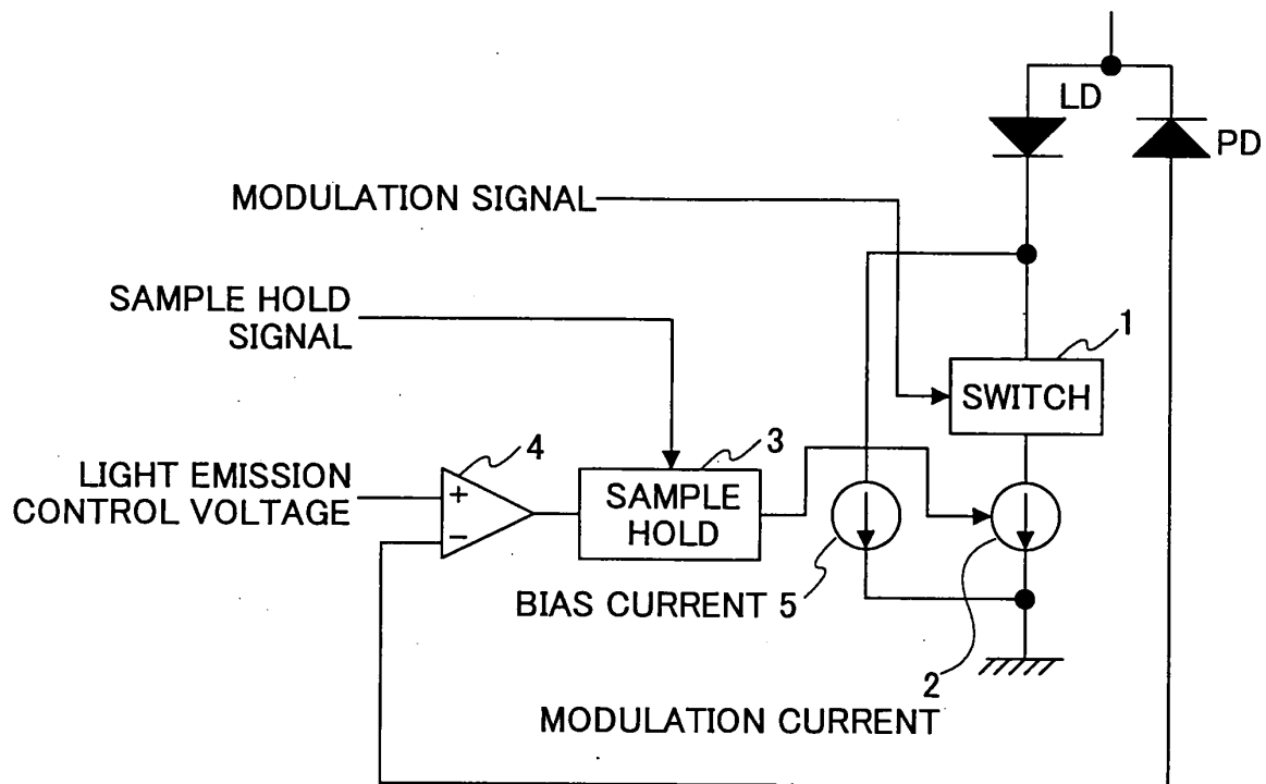
FIG.5 PRIOR ART
