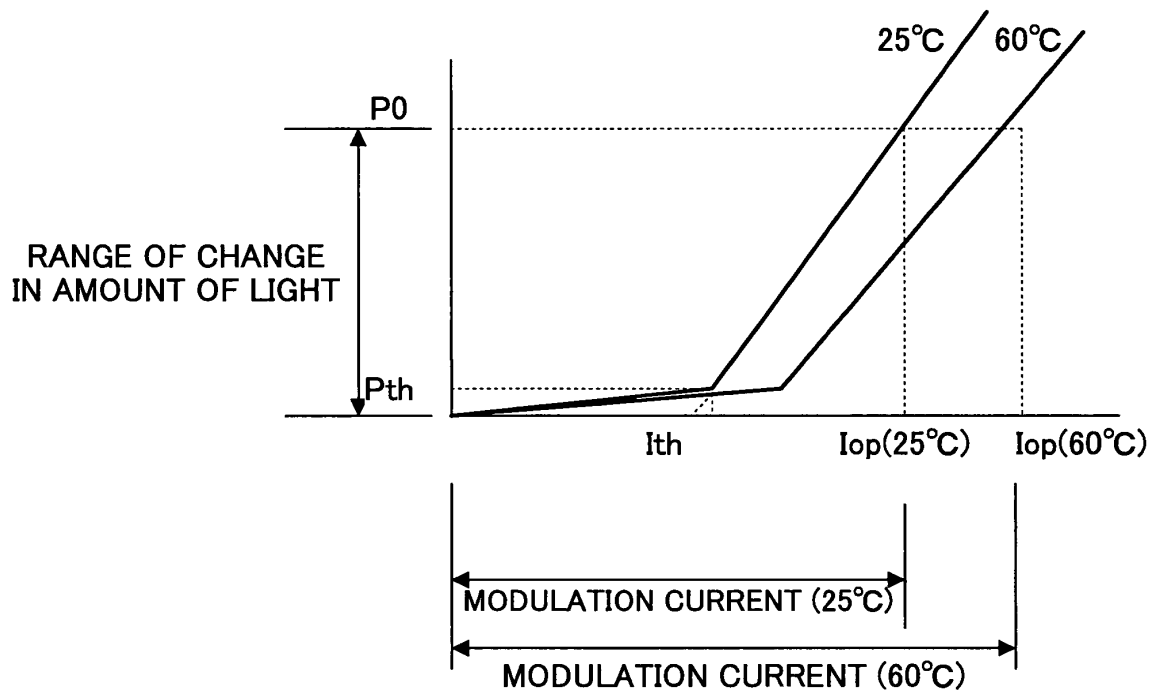
FIG.1 PRIOR ART
