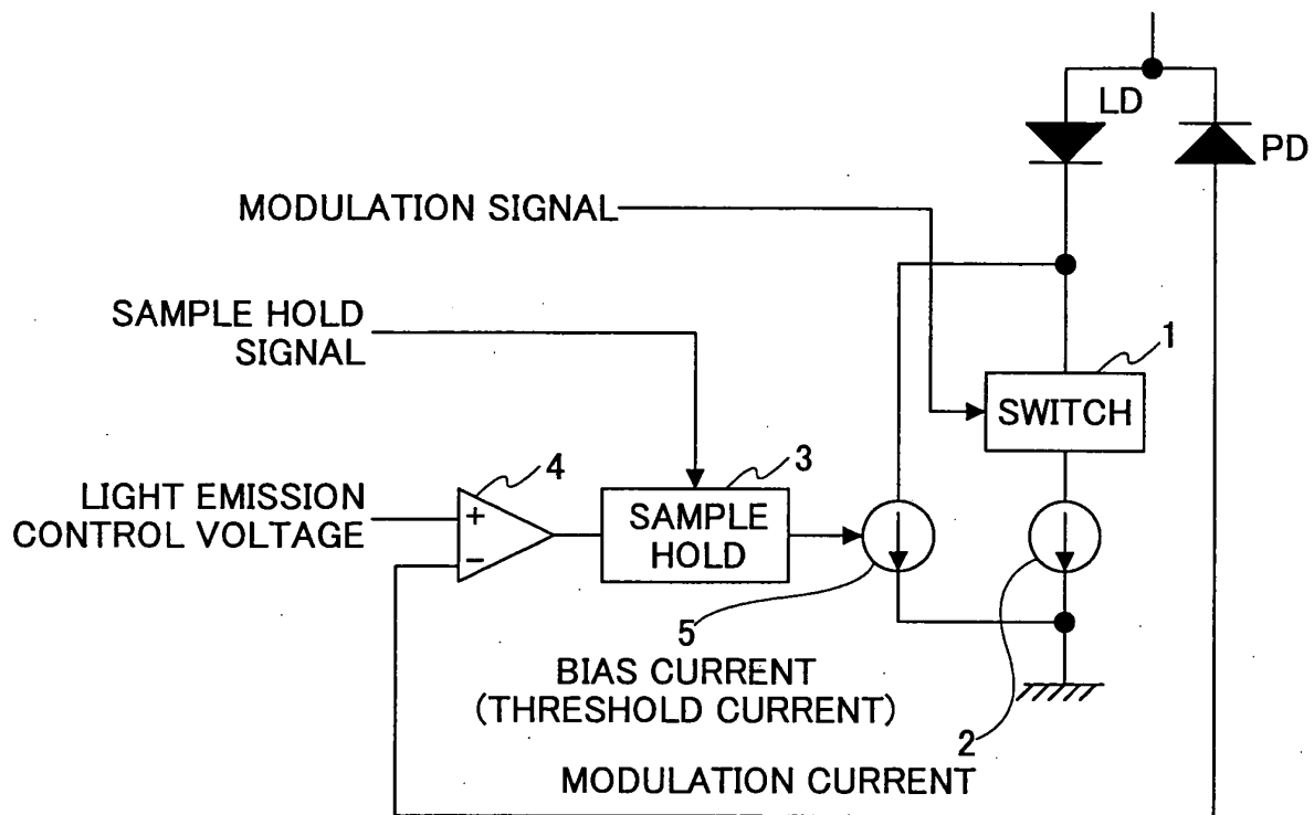
FIG.7 PRIOR ART
