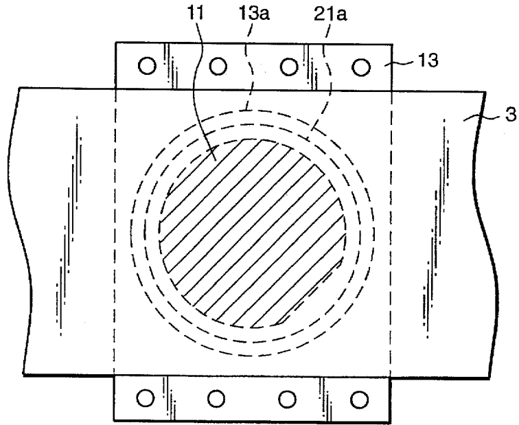
Fig. 2 (PRIOR ART)
