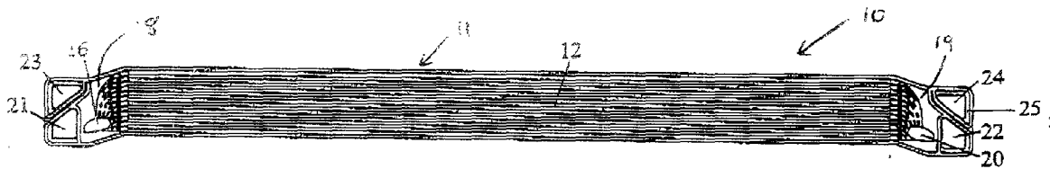
PRIOR ART FIG. 1b
