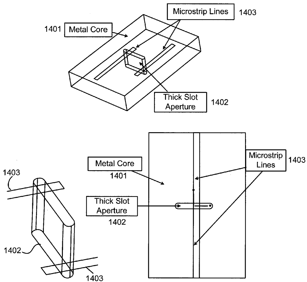
Figure 14: transparent view of a contactless interconnection.
