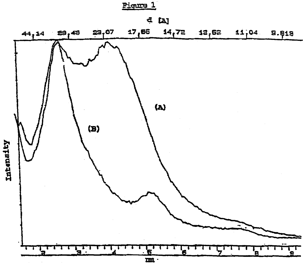
Figure 1: X-ray diffraction patterns of tallow methyl dihydroxyethylammonium montmorillonite expanded with PEG 6763 and containing (A) 60% clay and (B) 40% clay. X-ray reflections at 3.2 and 2.2 nm correspond to the fully expanded organoclay and partially expanded organoclay, respectively.
