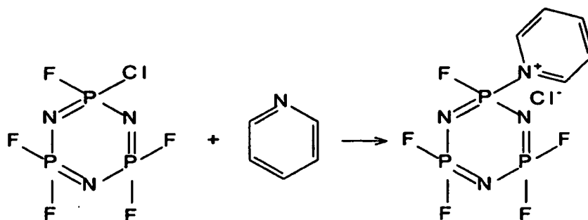
... Reaction scheme 3
