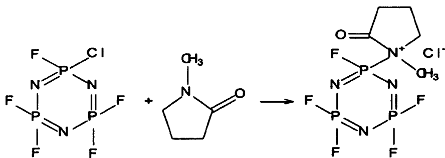
... Reaction scheme 2
