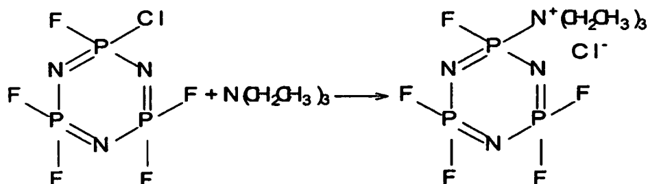
... Reaction scheme 1
