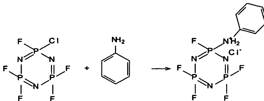
... Reaction scheme 4
