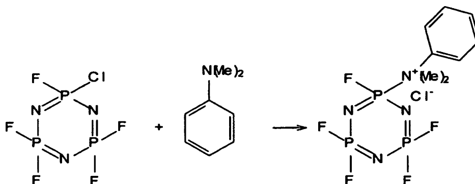
... Reaction scheme 5
