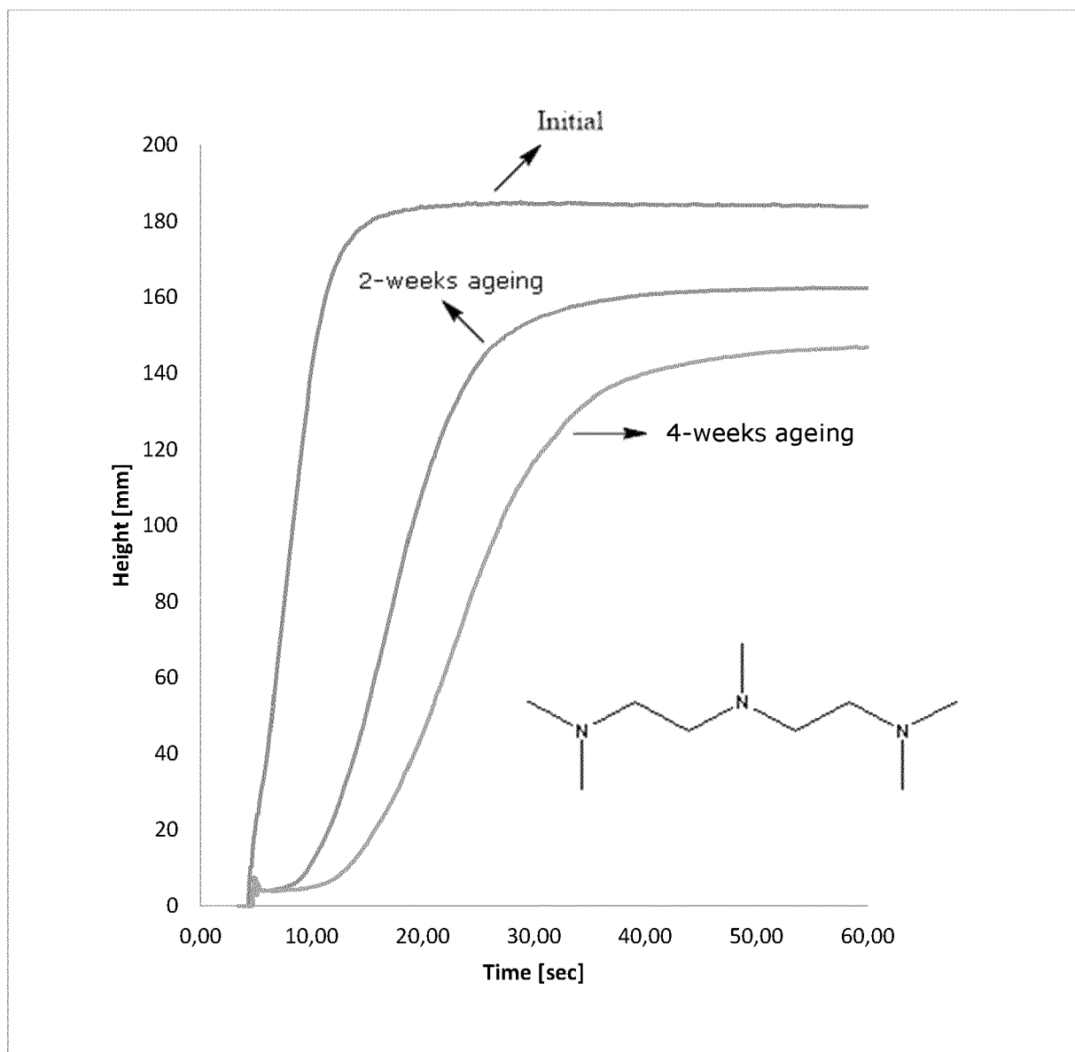
Figure 5: Rate of Rise profiles for foam made in accordance with Example 13 at 0 week, 2 weeks and 4 weeks
