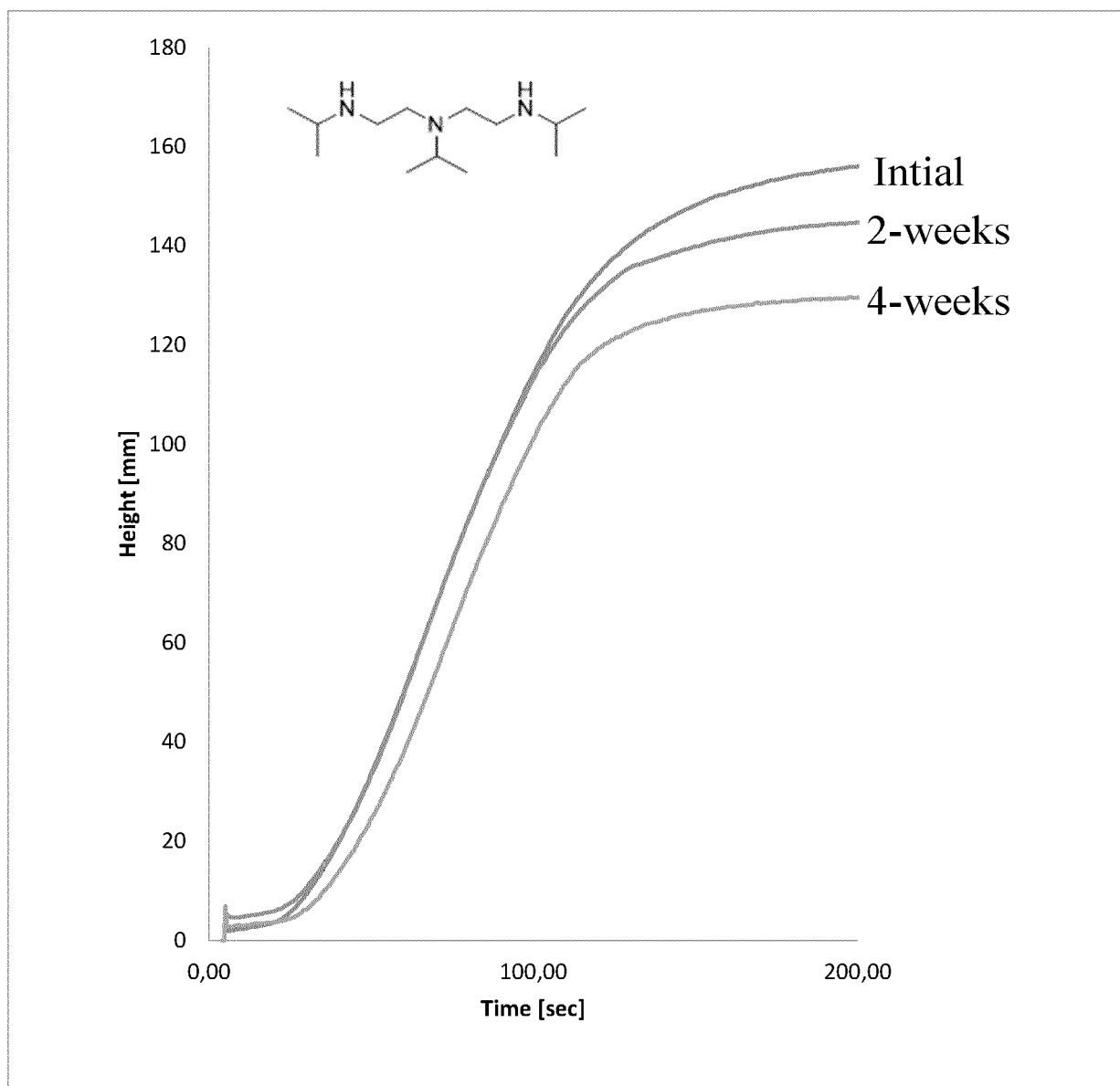
Figure 7: Rate of Rise profiles for foam made in accordance with Example 3 at 0 week, 2 weeks and 4 weeks
