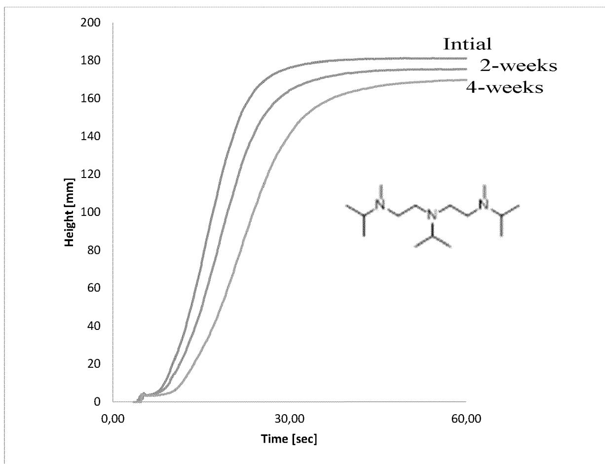
Figure 8: Rate of Rise profiles for foam made in accordance with Example 5 at 0 week, 2 weeks and 4 weeks
