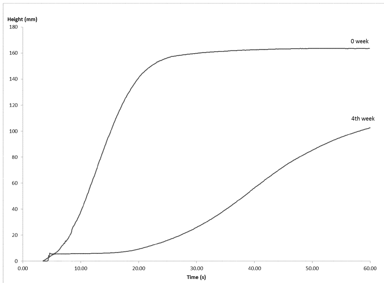
Figure 2: Rate of Rise profiles for foam made in accordance with Example 11 at 0 week and 4 weeks
