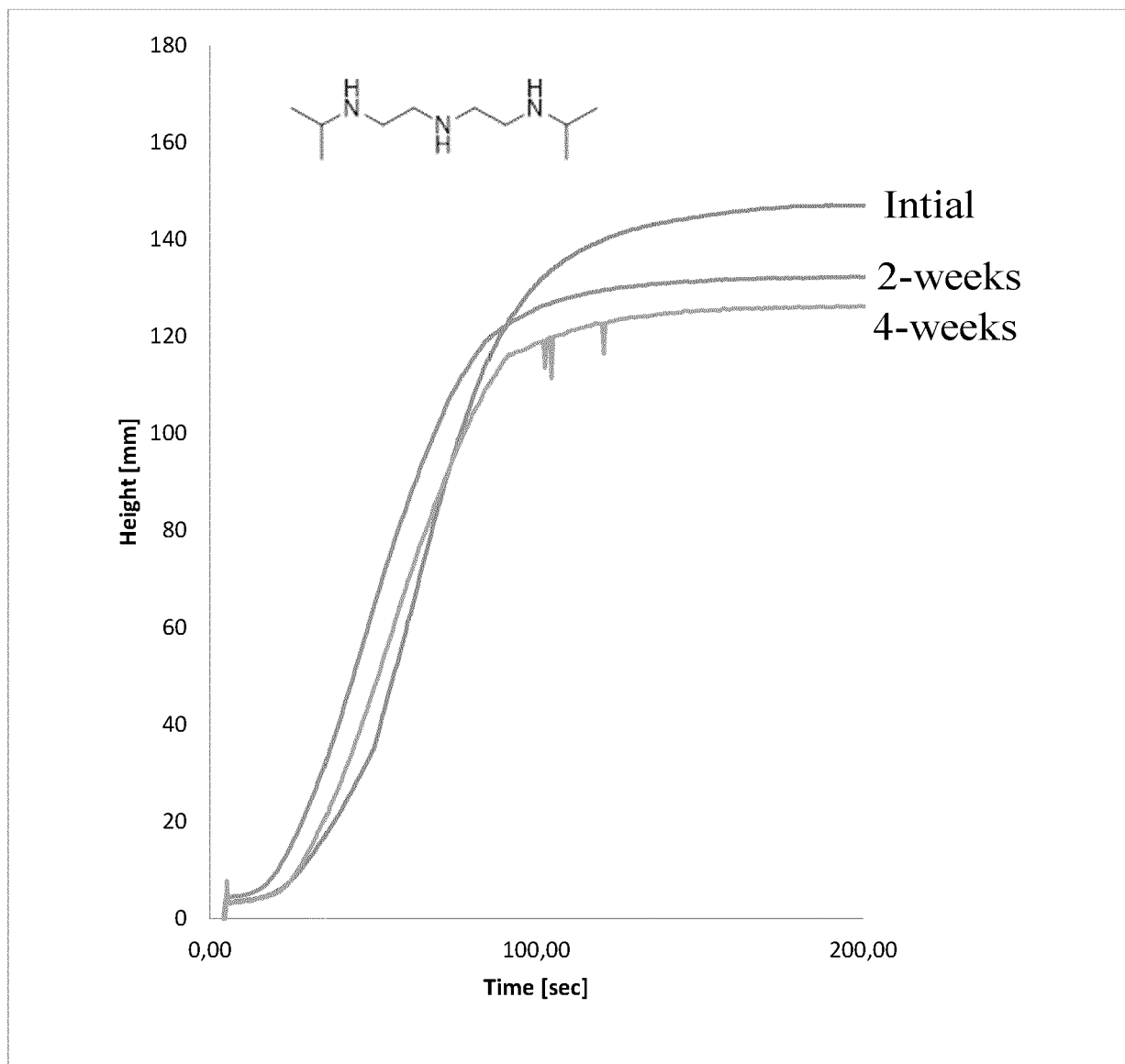
Figure 6: Rate of Rise profiles for foam made in accordance with Example 2 at 0 week, 2 weeks and 4 weeks
