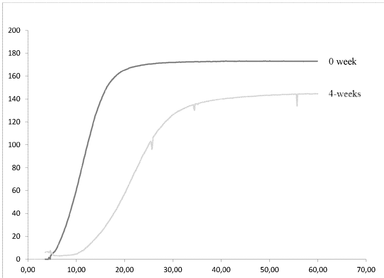
Figure 17: Rate of Rise profiles for foam made in accordance with Example 19 at 0 week and 4 weeks
