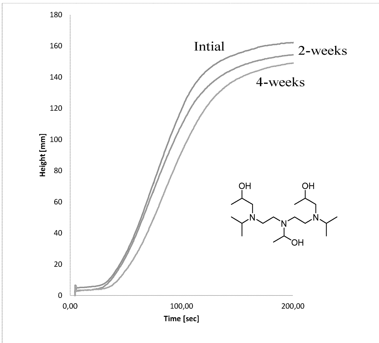
Figure 11: Rate of Rise profiles for foam made in accordance with Example 7 at 0 week, 2 weeks and 4 weeks
