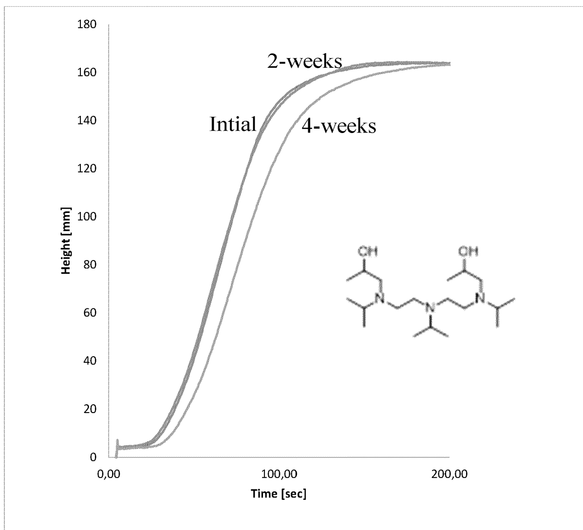
Figure 10: Rate of Rise profiles for foam made in accordance with Example 6 at 0 week, 2 weeks and 4 weeks
