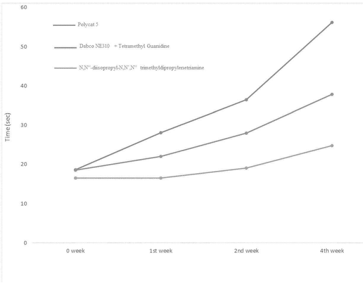
Figure 4: Time in seconds to 80% Maximum Height at 0 week, 1 week, 2 weeks and 4 weeks
