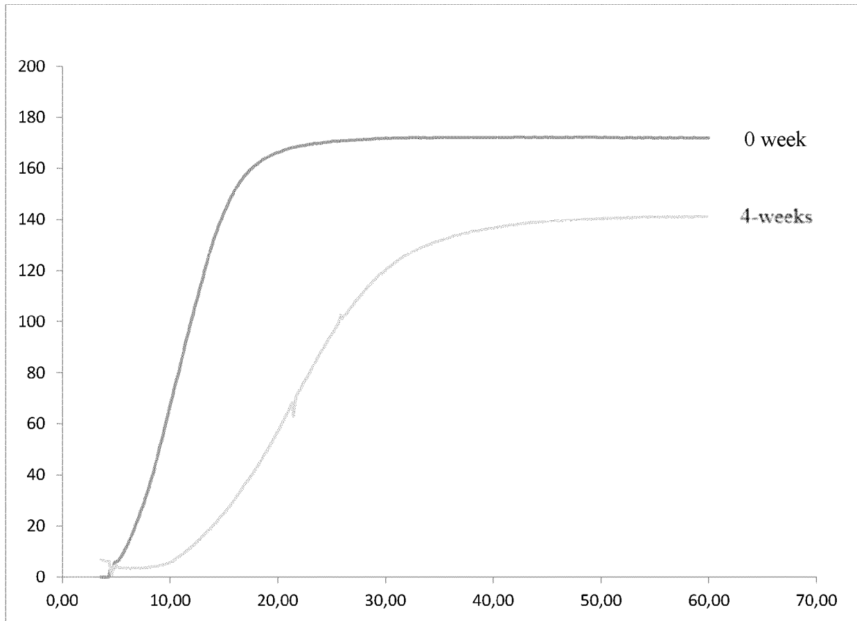
Figure 18: Rate of Rise profiles for foam made in accordance with Example 19 at 0 week and 4 weeks
