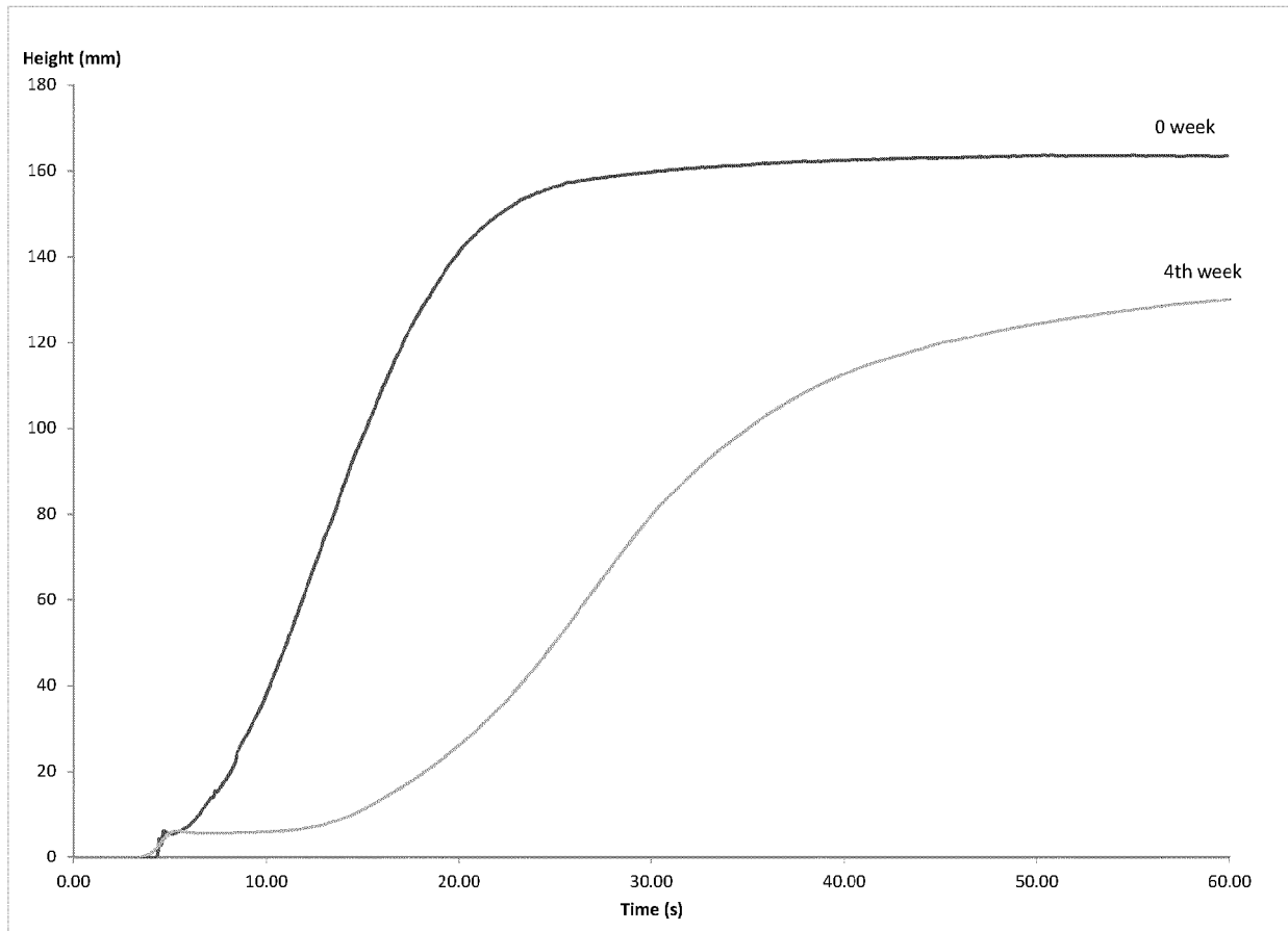
Figure 3: Rate of Rise profiles for foam made in accordance with Example 12 at 0 week and 4 weeks
