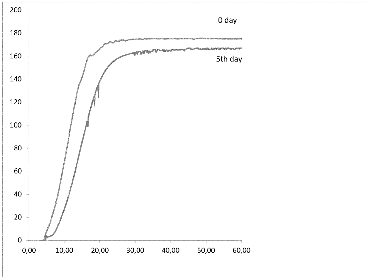
Figure 13: Rate of Rise profiles for foam made in accordance with Example 16 at 0 days and 5 days
