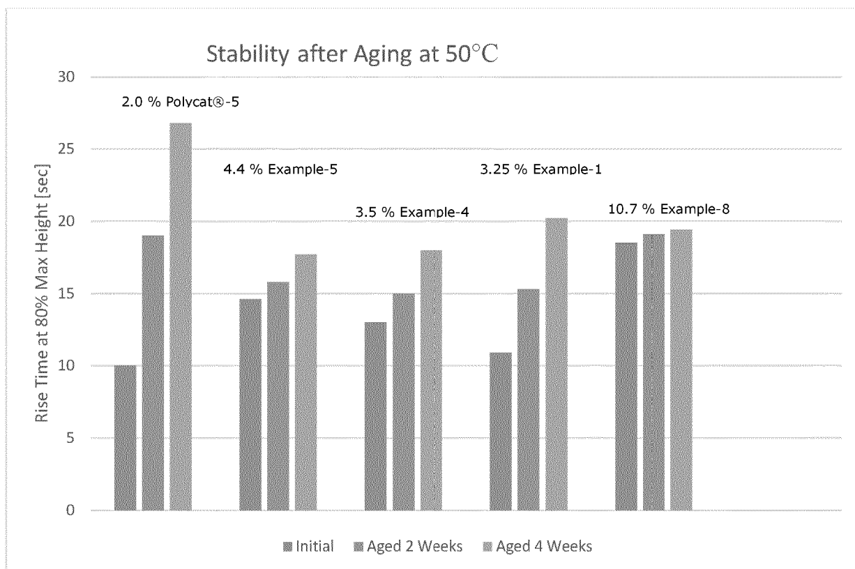
Figure 12: Stability after aging at 50 °C for the catalysts listed in Table 8
