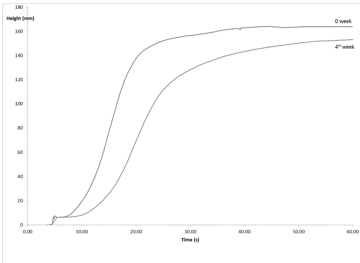
Figure 15: Rate of Rise profiles for foam made in accordance with Example 18 at 0 week and 4 weeks
