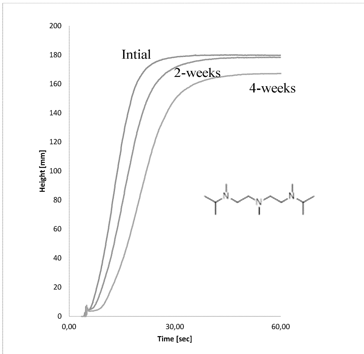
Figure 9: Rate of Rise profiles for foam made in accordance with Example 4 at 0 week, 2 weeks and 4 weeks
