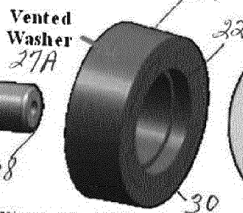
Close Up Views of Washer Vent Components
