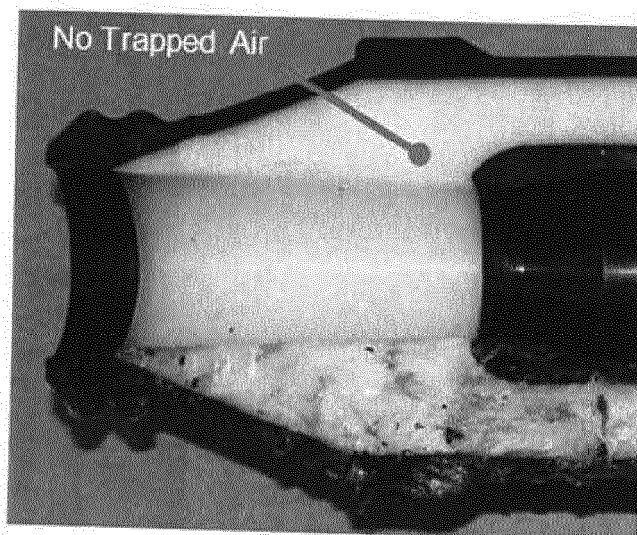
Splice Molded with Sintered Steel Core and Vacuum
