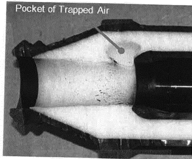
Splice Molded with Sintered Metal Vents
