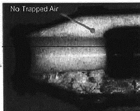
Figure 6 Splice Made with Pin Vent and Vacuum
