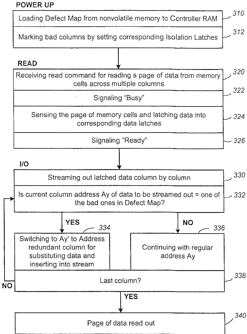
READ OPERATION (Prior Art)
