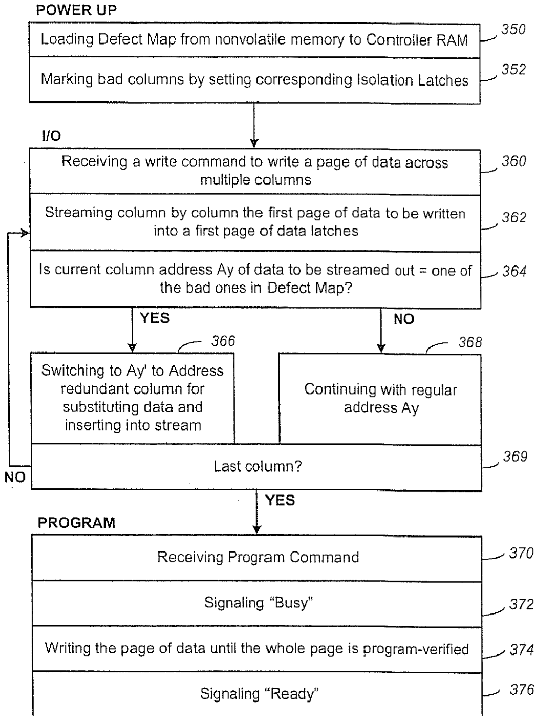
PROGRAM OPERATION (Prior Art)
