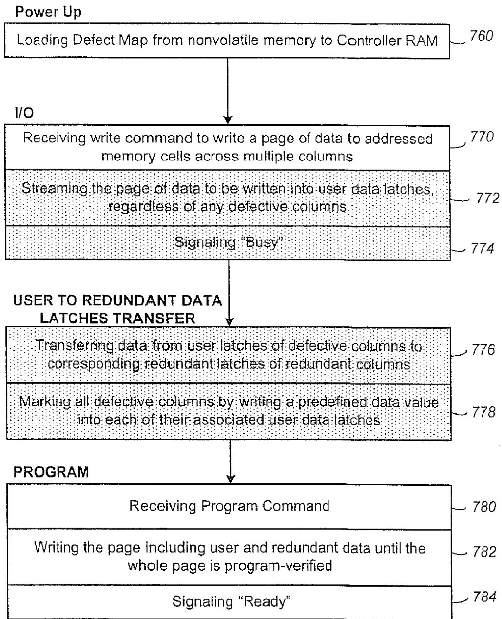
WRITE OPERATION USING REDUNDANT DATA BUFFERED IN DATA LATCHES OF DEFECTIVE COLUMNS
