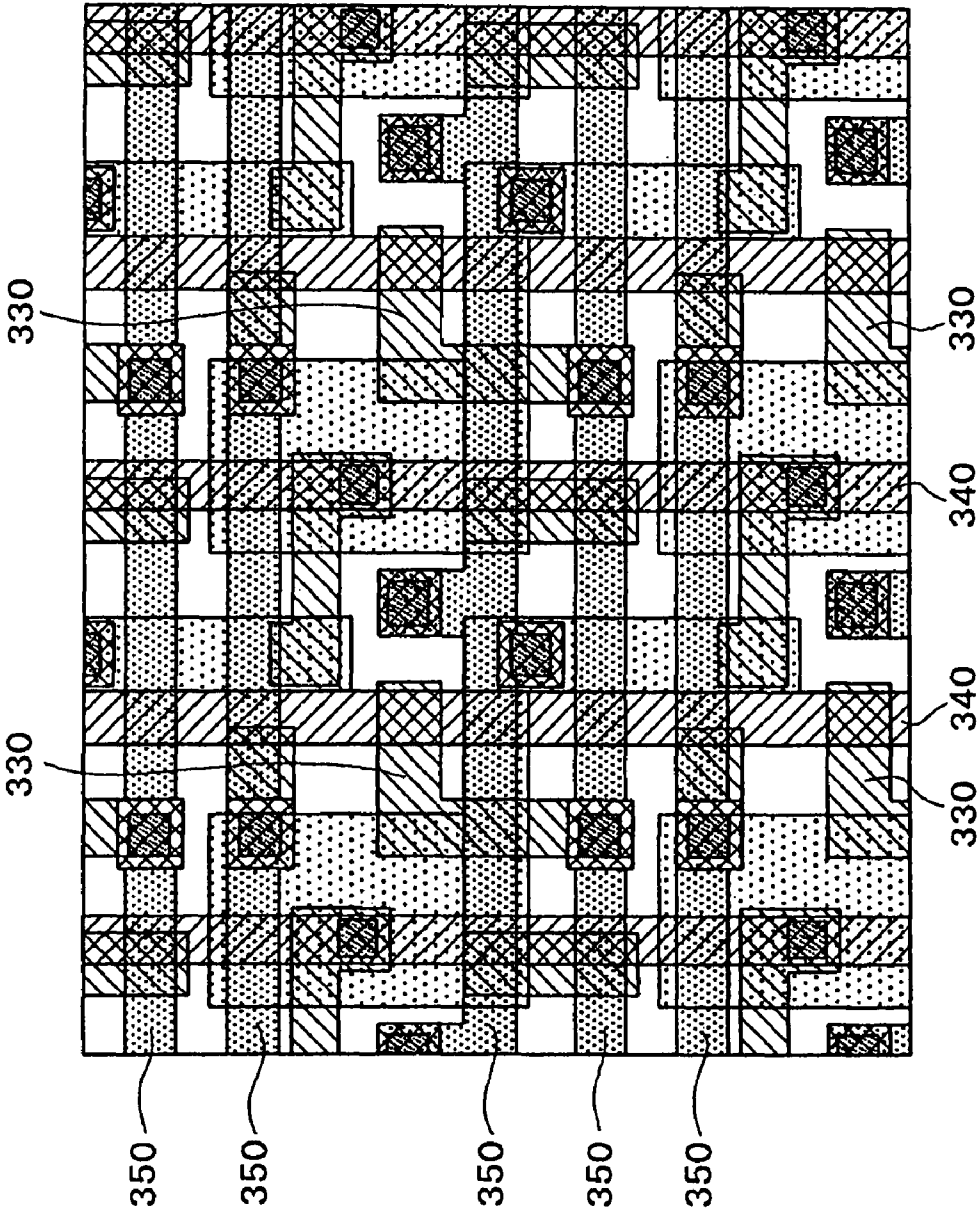
FIG. 4 METALLIC WIRING, INTER-WIRING CONTACT, AND ACTIVE REGION
