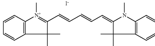
Hexamethylindodicarbocyanine iodide (HIDCI)
