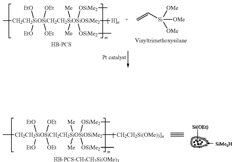
Scheme 2
