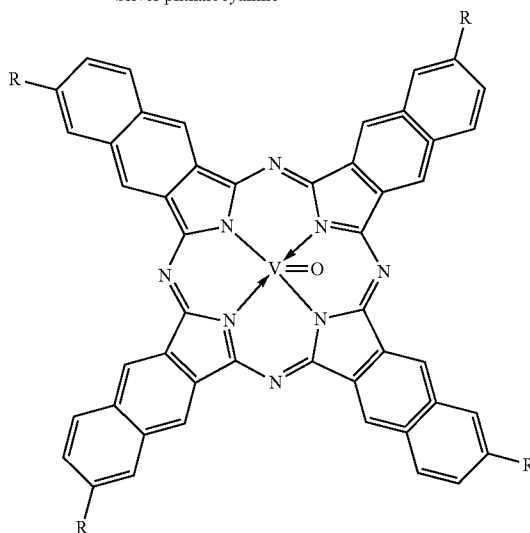
Vanadyl naphthalocyanine I -
