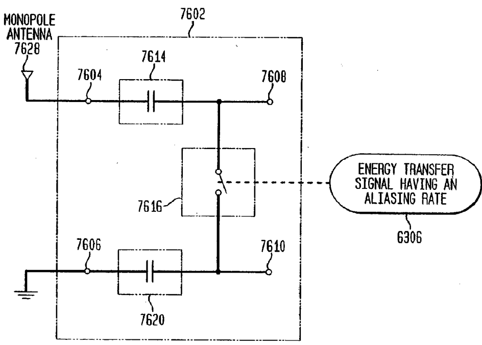
FIG. 76C SINGLE INPUT TO DIFFERENTIAL OUTPUT
