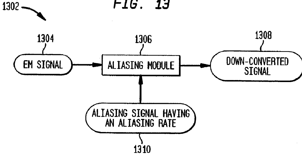
GENERIC DOWN-CONVERTING SYSTEM
