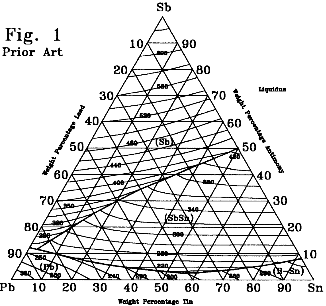
Ternary Antimony-Tin-Lead phase diagram.
