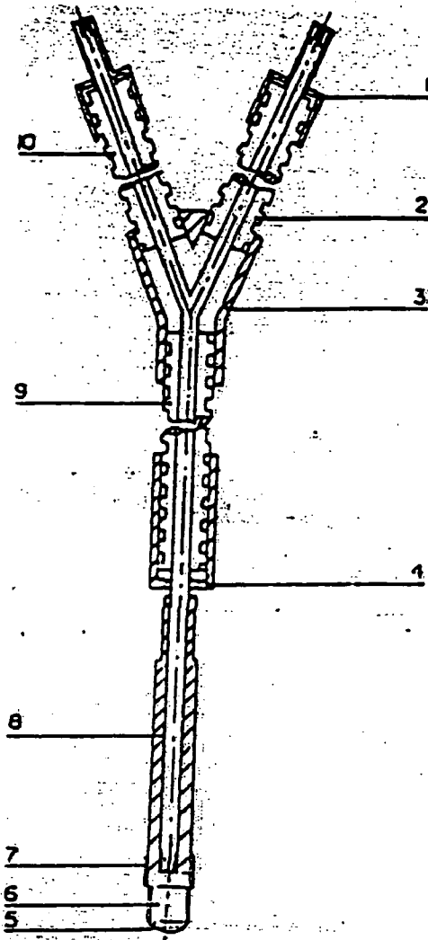
Figure : Configuration of the Fiber Optic Temperature Switching Immersion Probe
