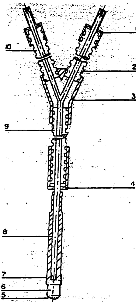
Configuration of the Fiber Optic Temperature Switching Immersion Probe
