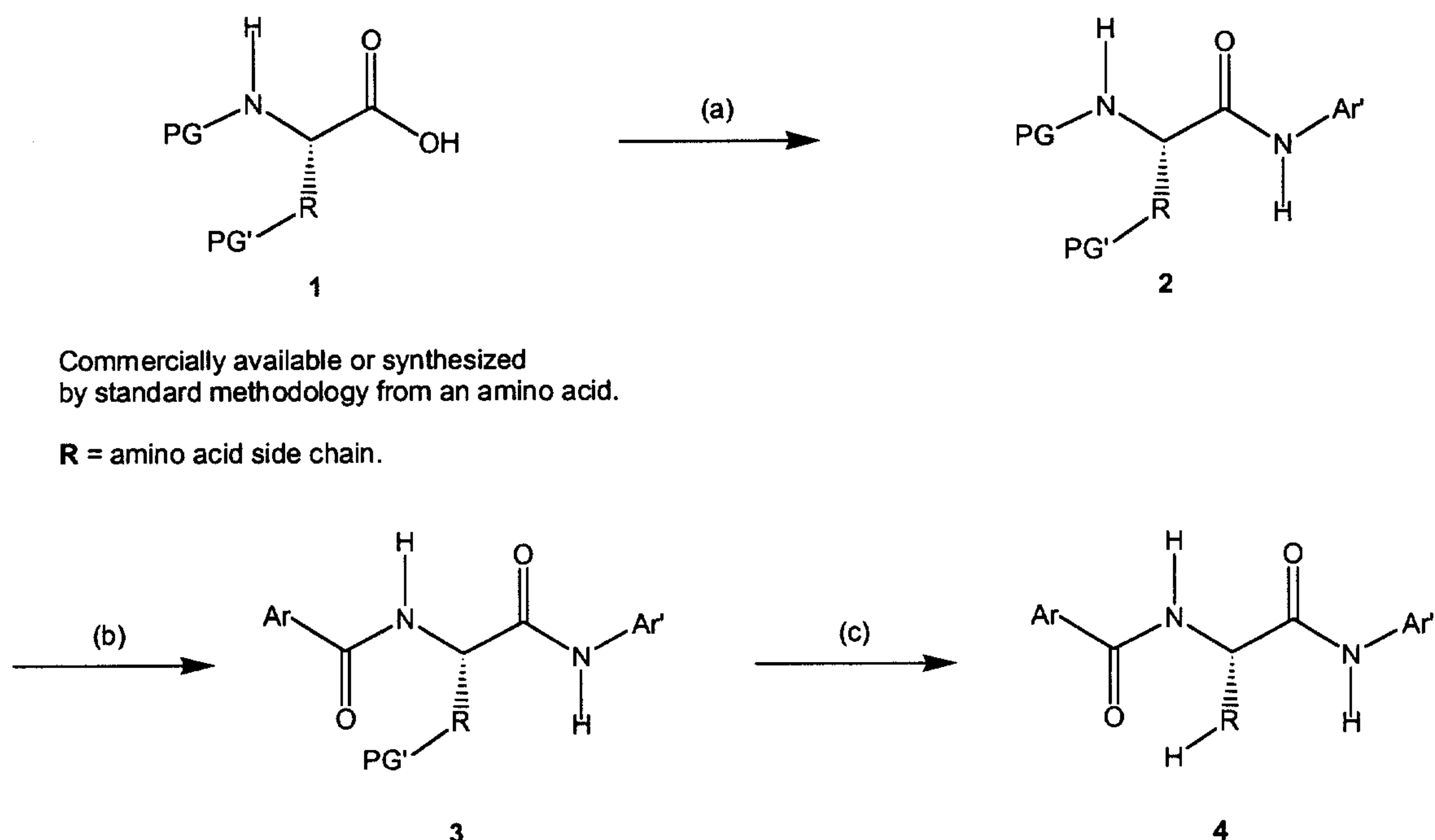
Scheme 1: General example showing sequential addition of Ar'-NH 2 followed by Ar-CO 2 H.
