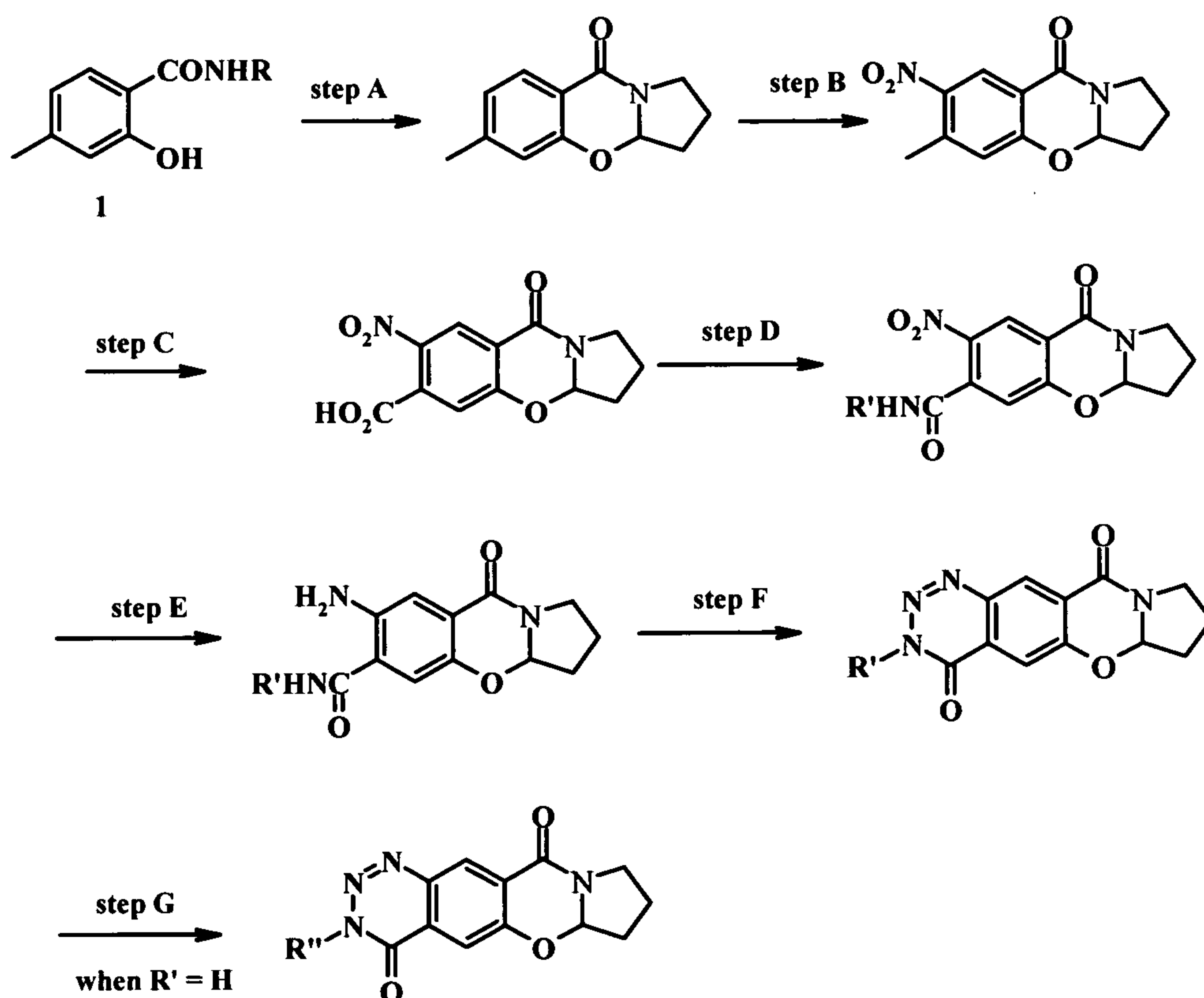
SCHEME 2
