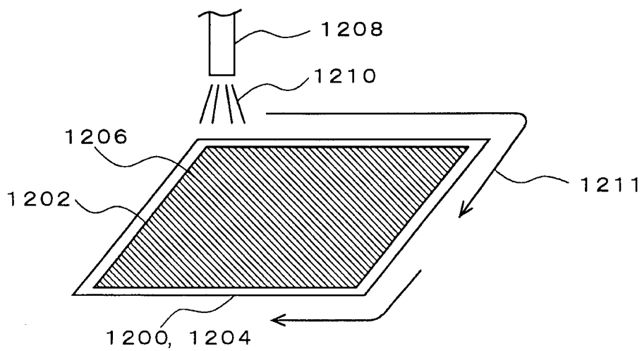
FIG. 108c (Prior Art)
