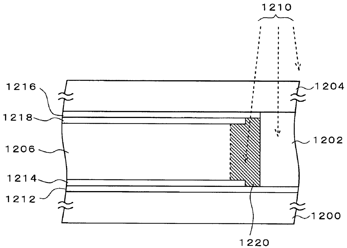
FIG. 109 (Prior Art)
