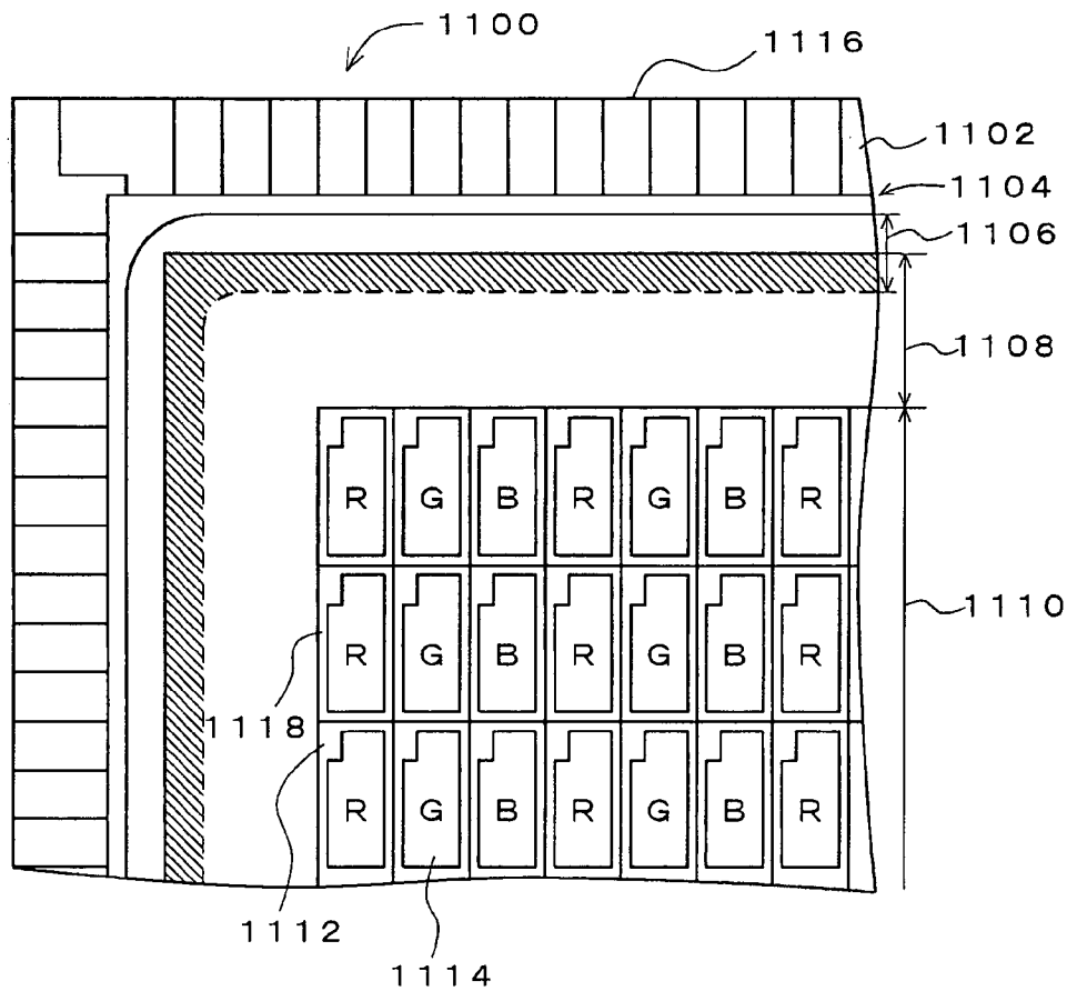
FIG. 104 (Prior Art)
