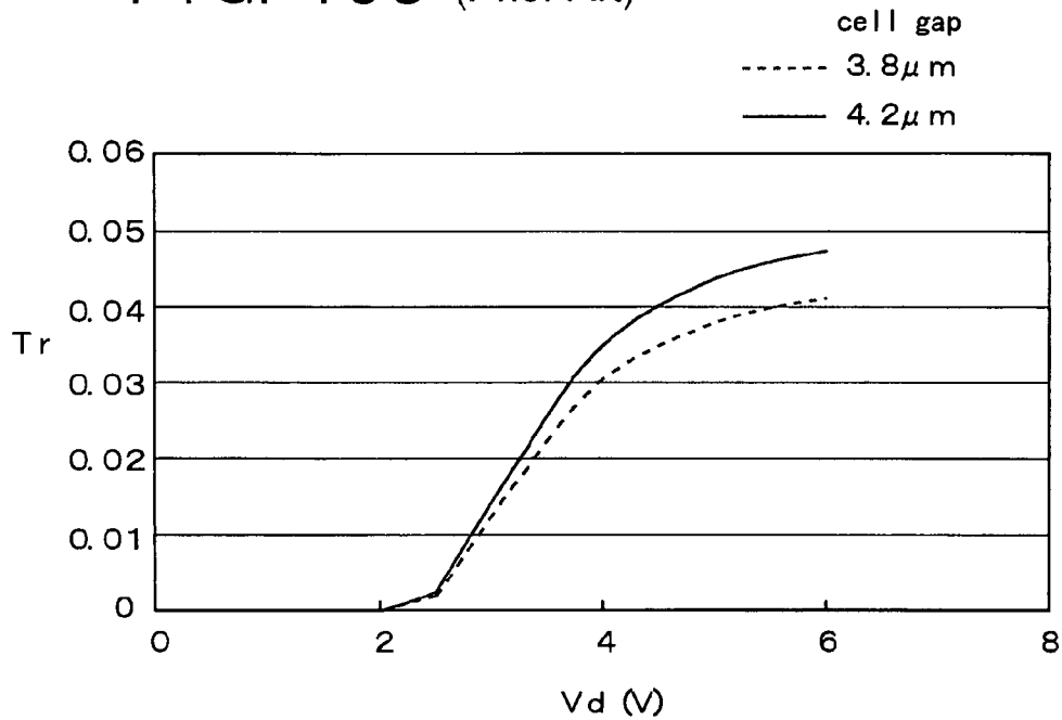
FIG. 103 (Prior Art)
