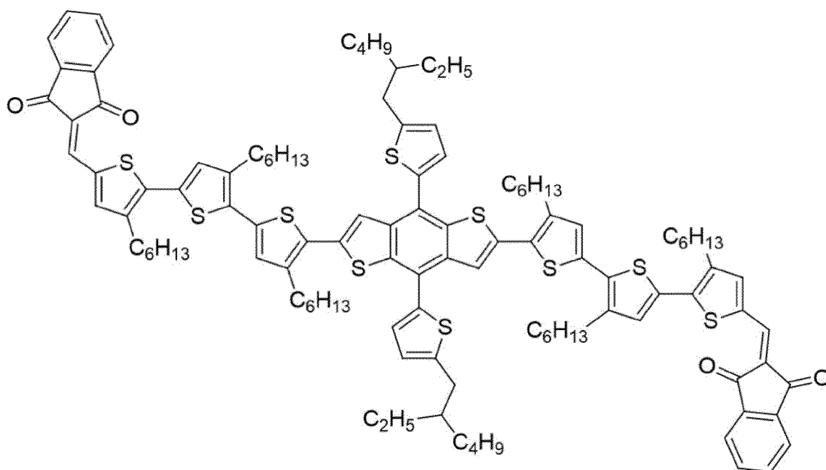
Exemplary Compound 8
