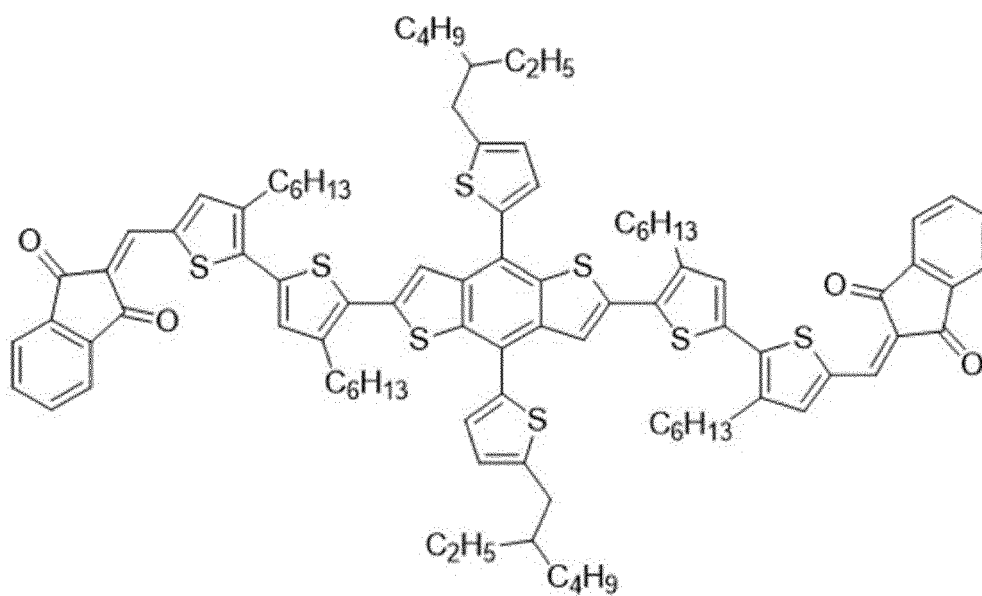
Exemplary Compound 1
