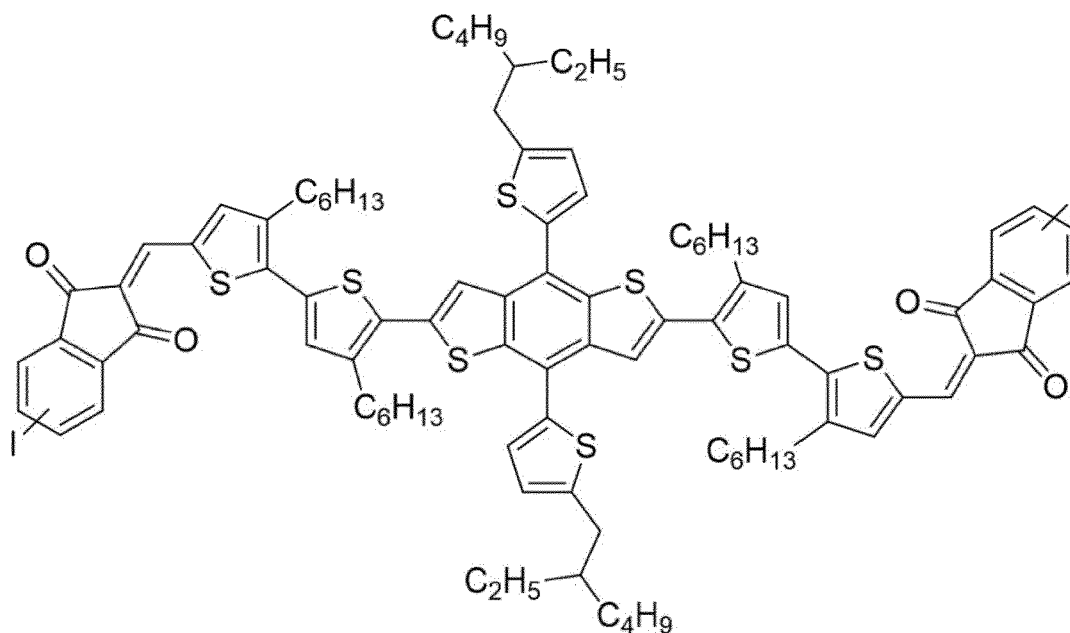
Exemplary Compound 7
