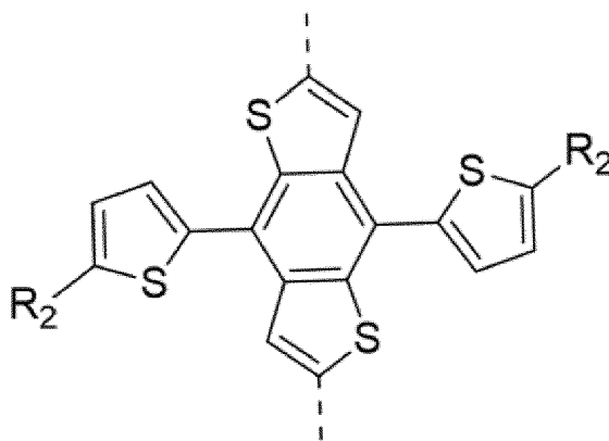
General Formula (2)
