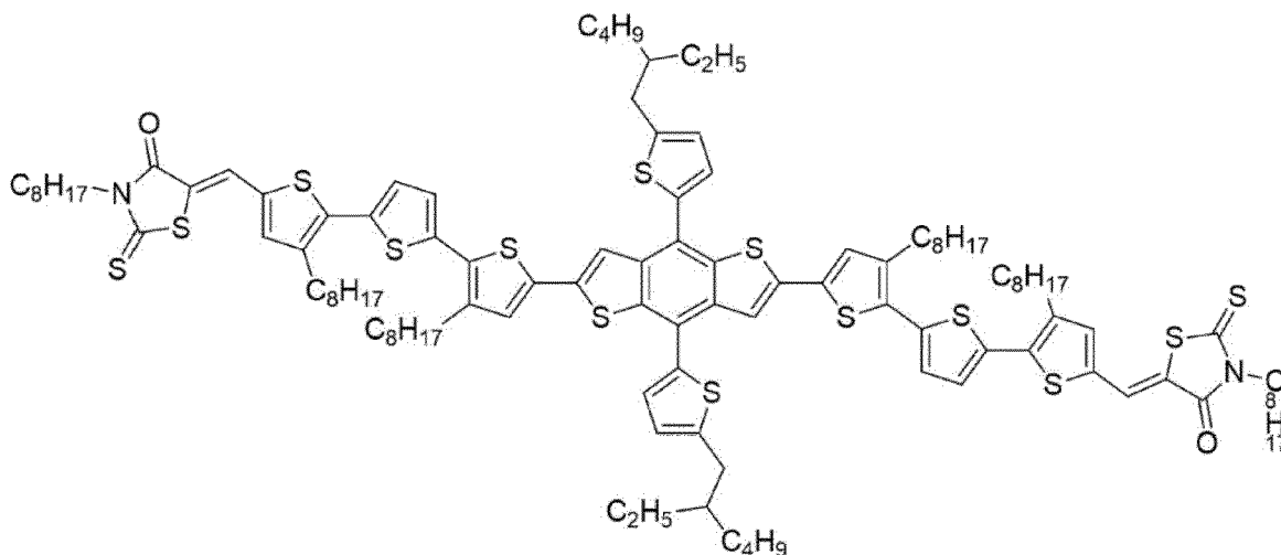
Exemplary Compound 4
