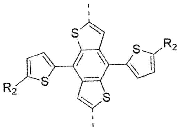
General Formula (2)
