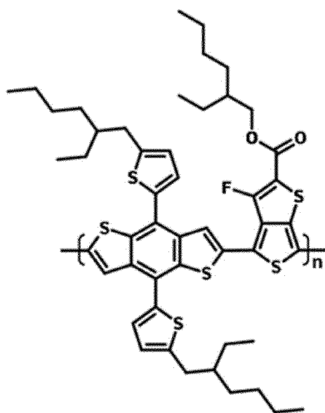
General Formula (12)
