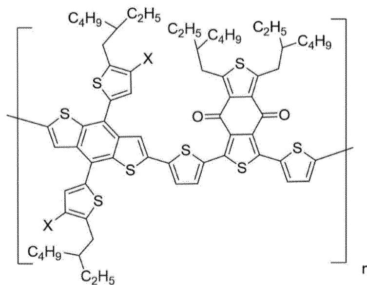
General Formula (13)
