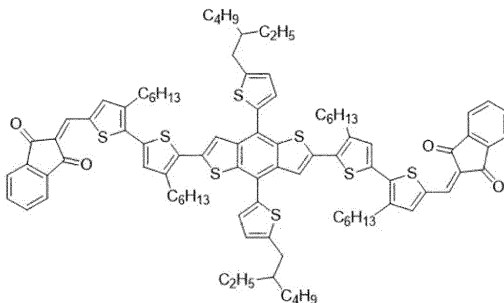
Exemplary Compound 1
