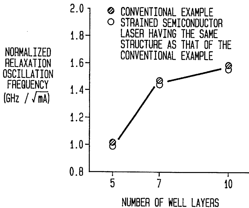
FIG. 8 (PRIOR ART)
