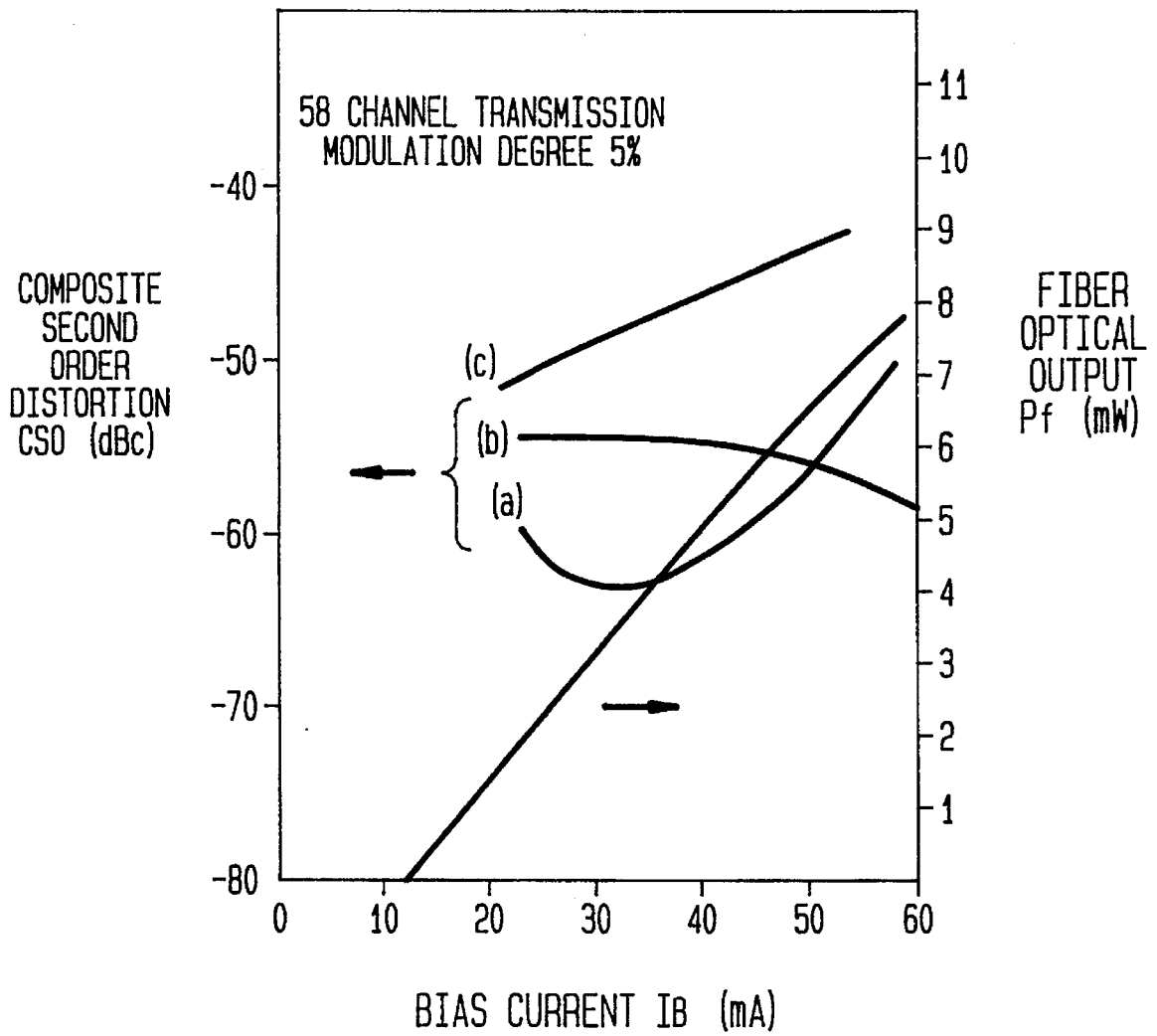
FIG. 9 (PRIOR ART)
