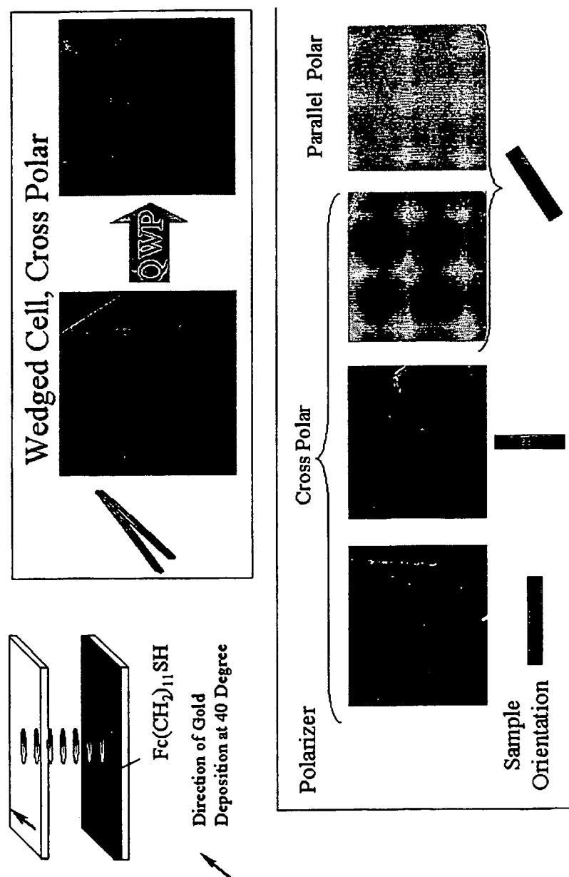
FIG. 17 Ferrocene-terminated SAM Template Azimuthal Orientation of 5CB Parallel to the Gold Topology of the Substrate
