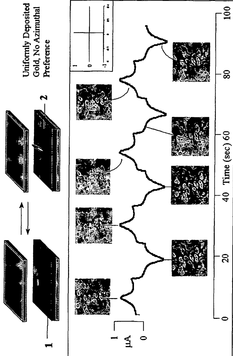
FIG. 16 In situ Electrochemical Control of Switching the Orientation of Liquid Crystal
