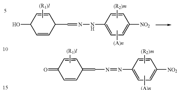
Reaction Scheme 2
