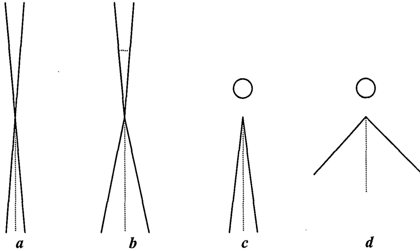
Figure 9. Representative Flow Patterns From Various Mixer Designs. a) Wedge Mixer, b) Sawtooth Tab Mixer, c) Air Injection Mixer With Air Off, d) Air Injection Mixer With Air On (0.16 lb m /s).
