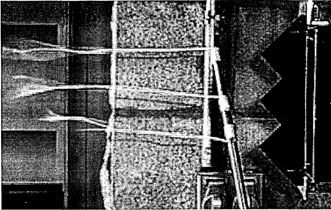
Figure 6. Flow Behind the Sawtooth Tab Mixer
