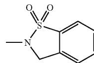
2,3-dihydro-tenzo[d]isothiazole-1,1-dioxide-2-yl
