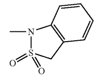
1,3-dihydro-benzo[c]isothiazole-2,2-dioxide-1-yl
