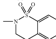
3,4-dihydro-2H-benzo[e][1,2]thiazine-1,1-dioxide-2-yl
