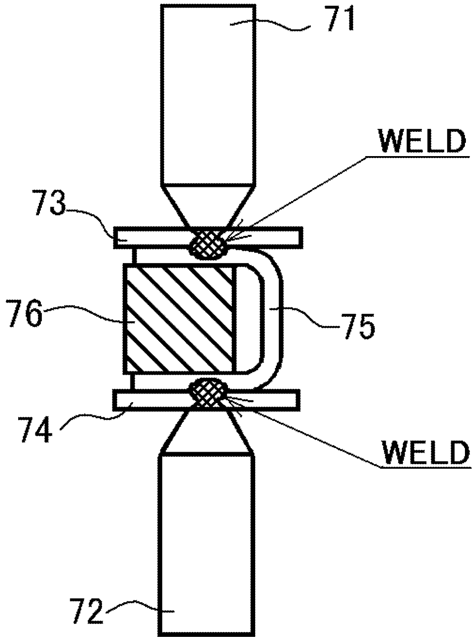
FIG. 11 (PRIOR ART)
