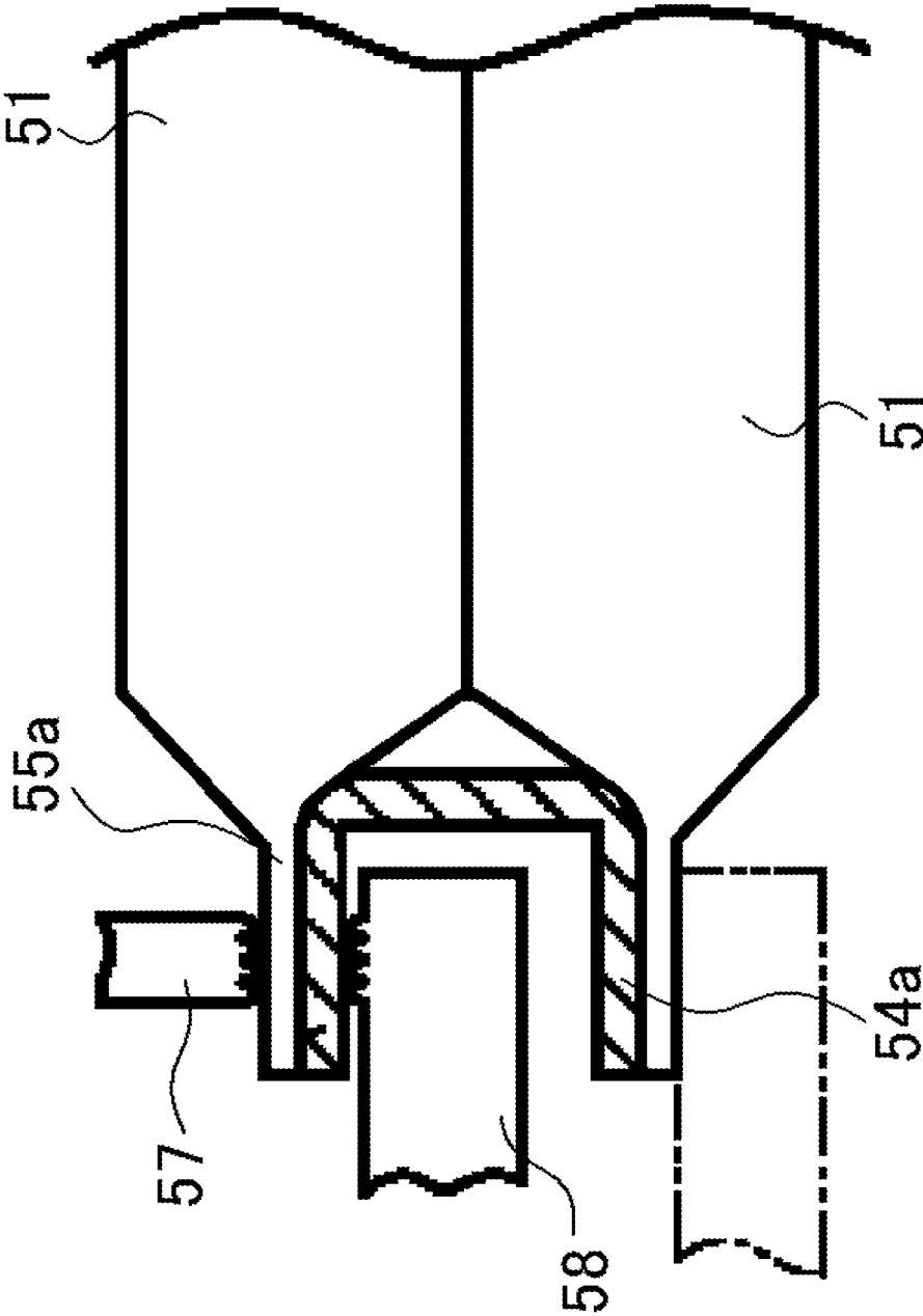
FIG.10 (PRIOR ART)
