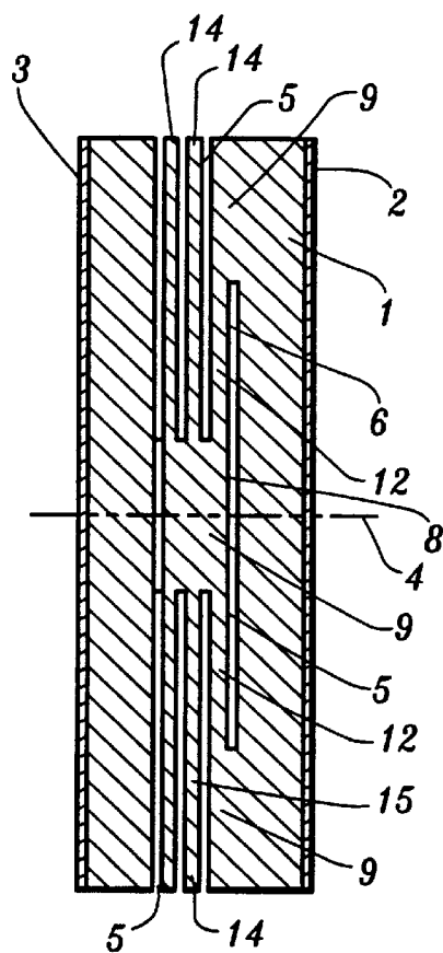
FIG. 3 (PRIOR ART)
