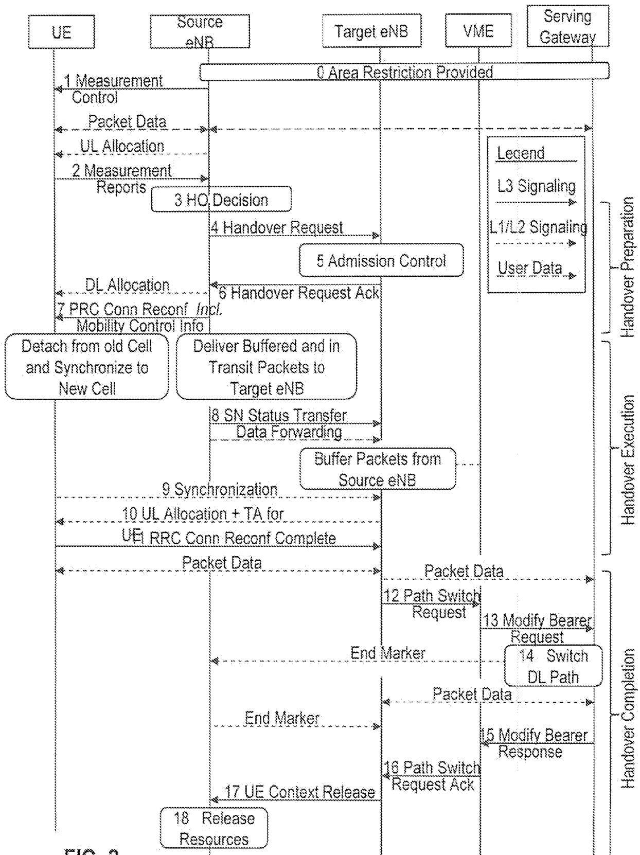
FIG. 2 PRIOR ART
