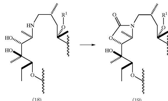
Scheme 13
