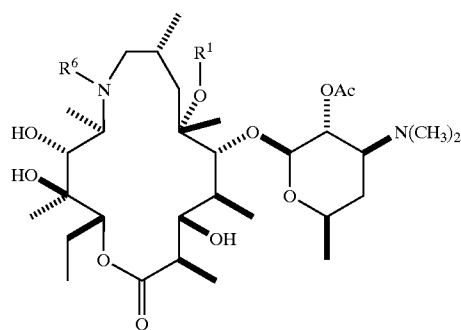
Scheme 10
