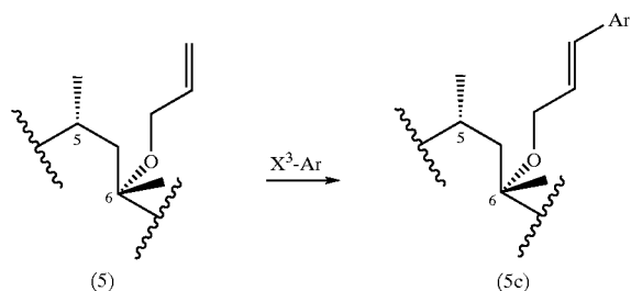
21 Scheme 5
