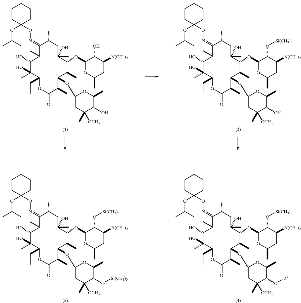
Scheme 1
