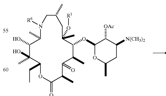
Scheme 11
