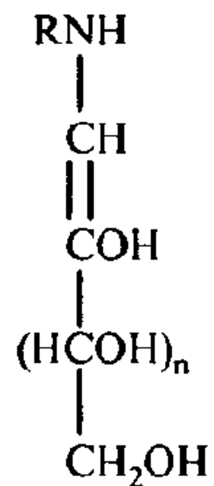
Enol form
