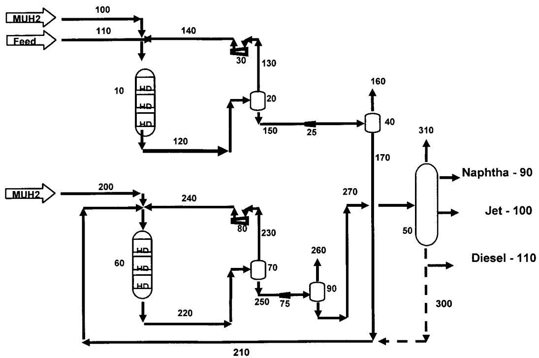
FIG.1 Two Stage Process
