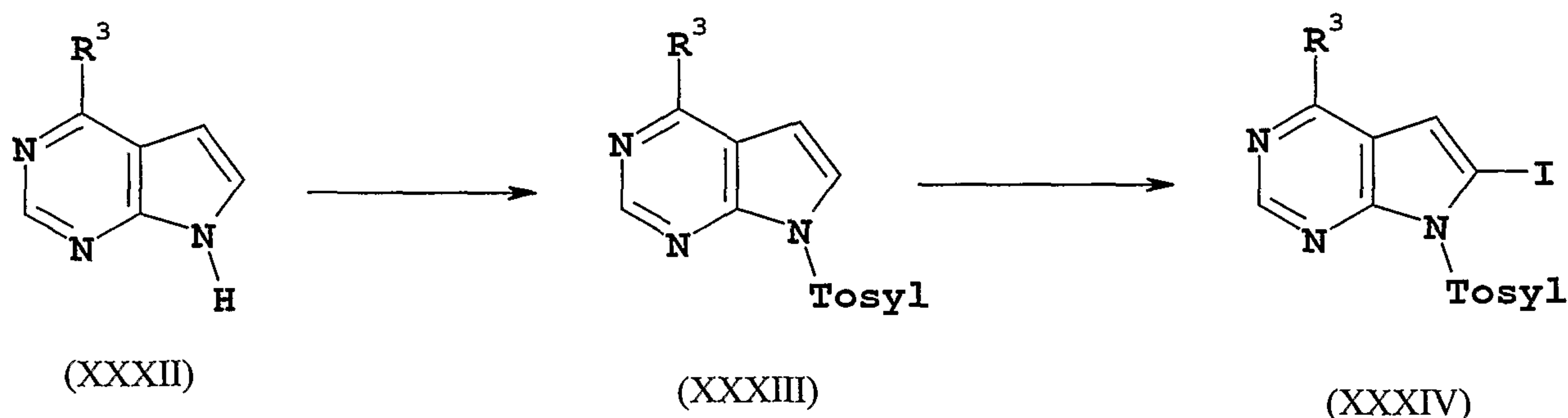
SCHEME 1
