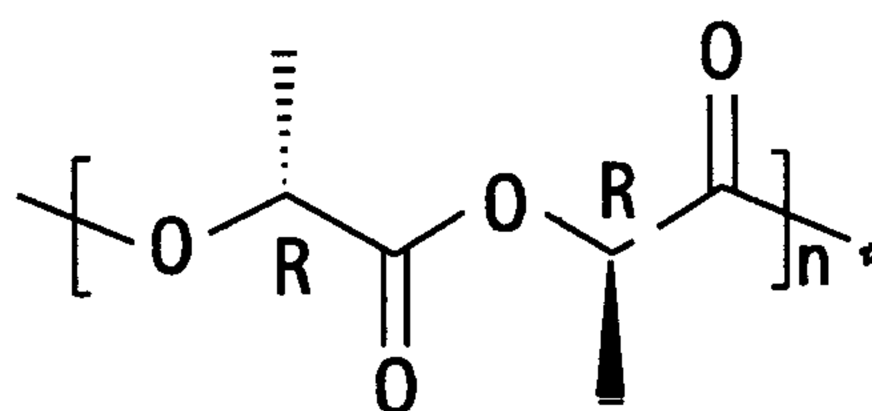
poly (D-lactide)
