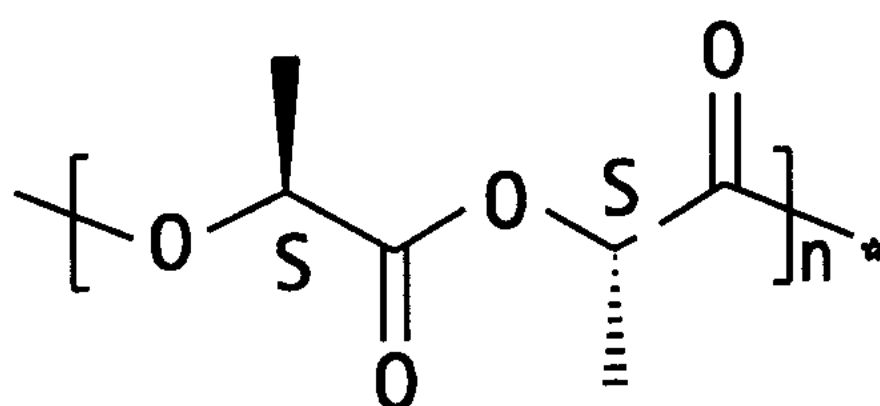
poly (L-lactide)
