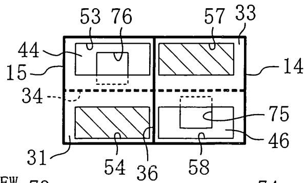
FIG. 11 (A) VIEW TAKEN IN DIRECTION OF ARROWS X-X
