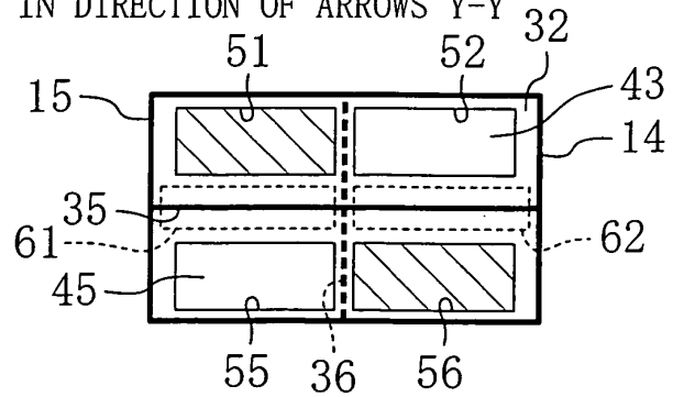
(C) VIEW TAKEN IN DIRECTION OF ARROWS Y-Y
