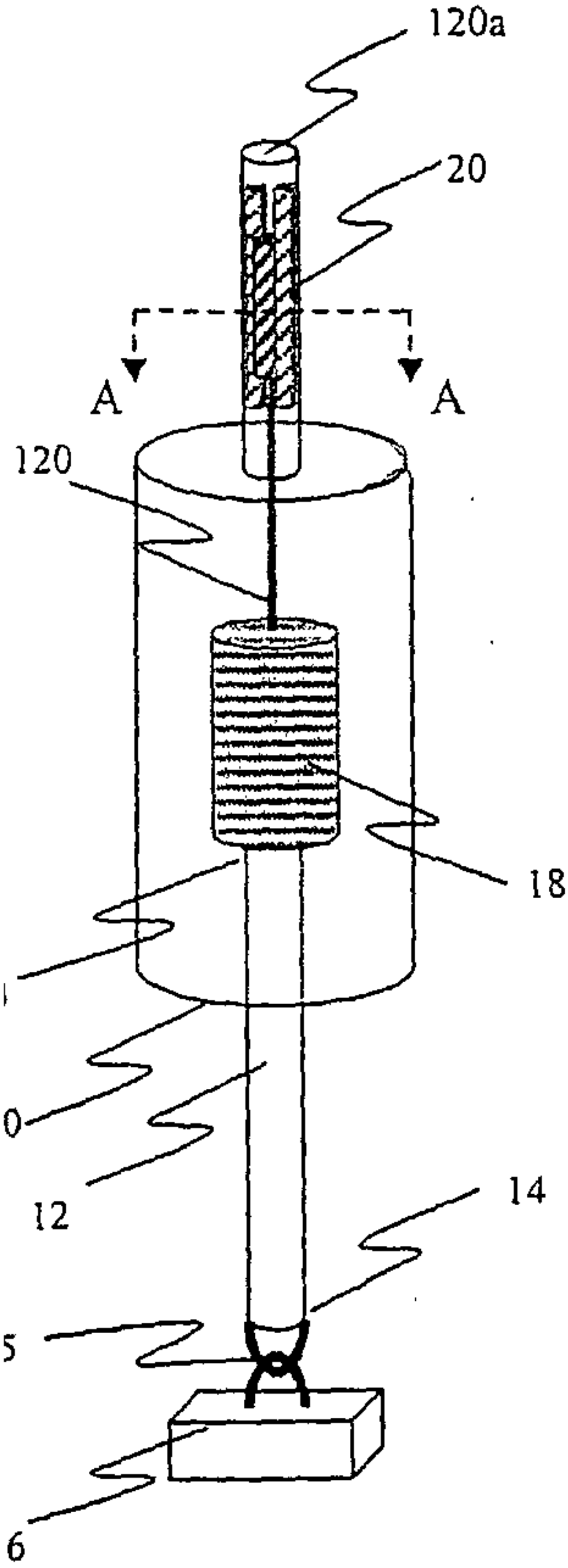
FIGURE 1A Anchored WEC w/LEG "Configuration A"
