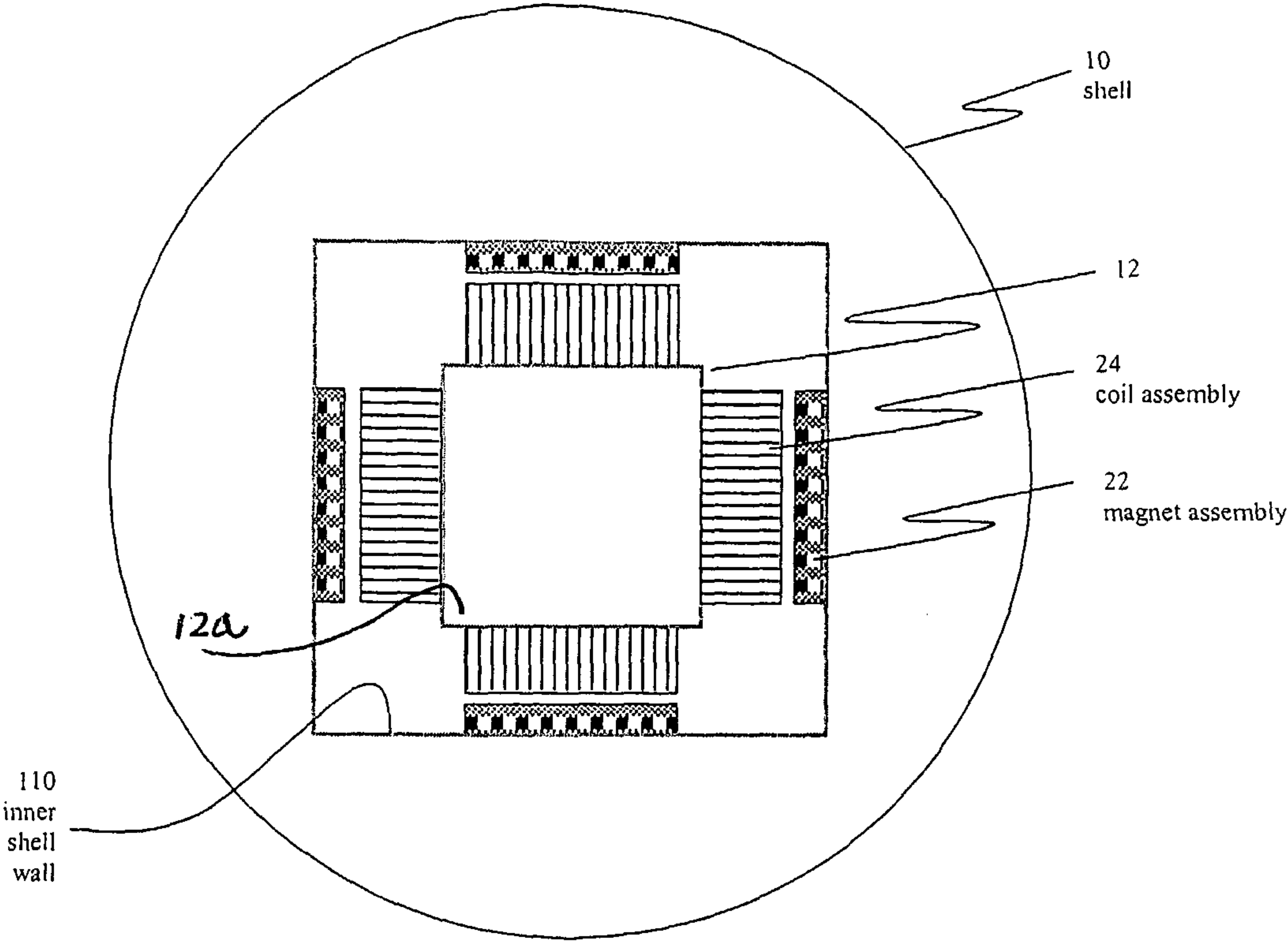
FIGURE 1B1 Cross-sectional View of Four-sided LEG
