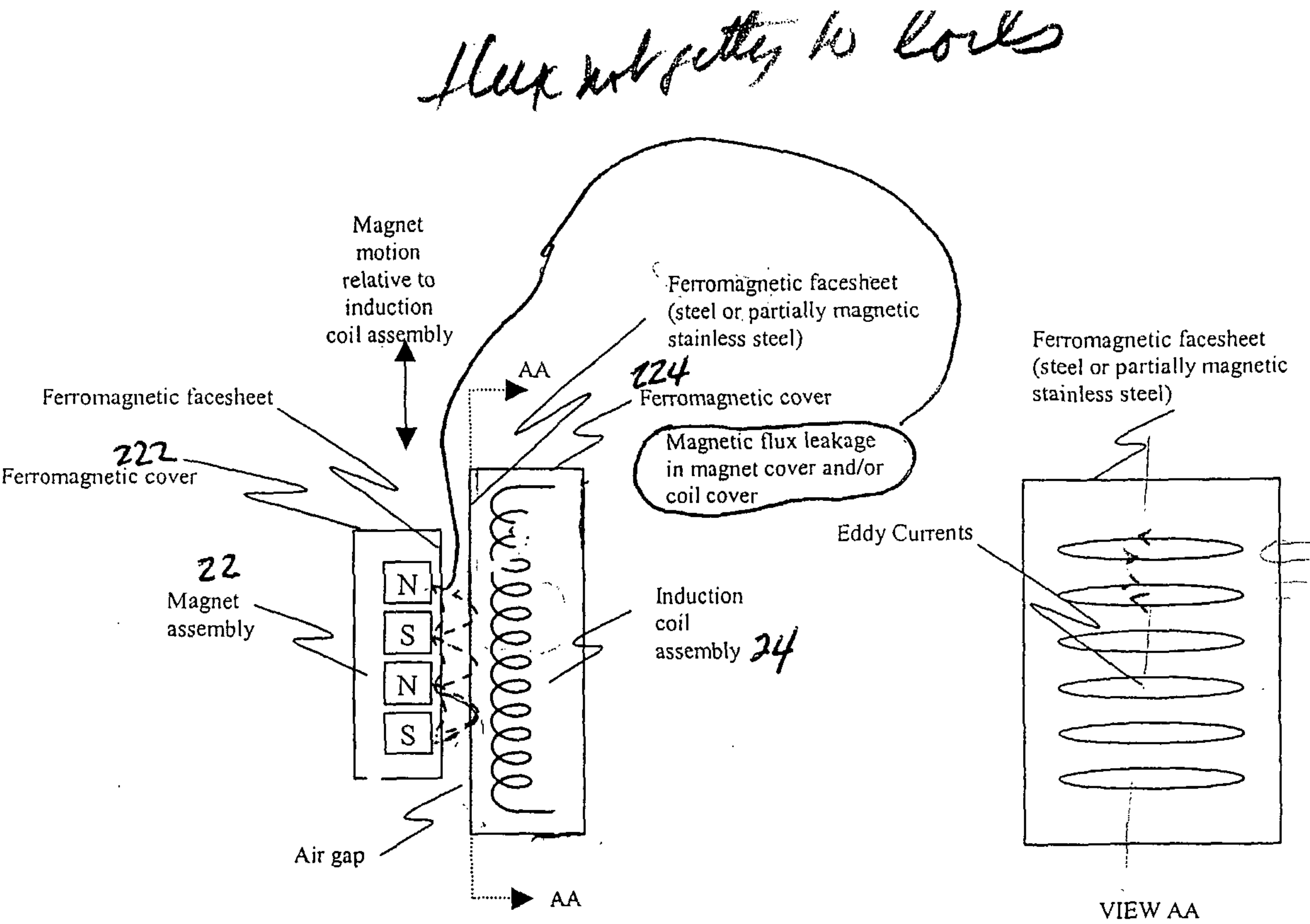
FIGURE 11 Waterproof Encapsulation with Eddy Current Losses
