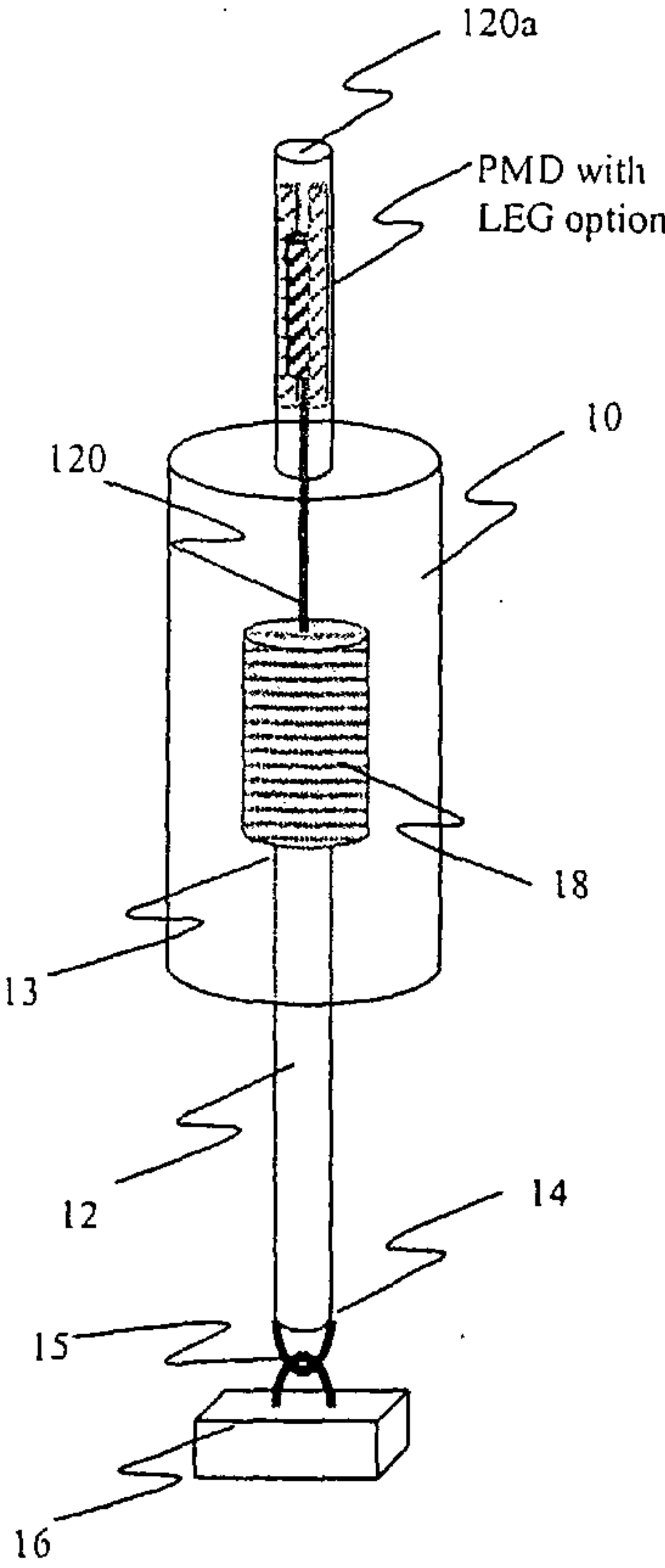
FIGURE 8A Anchored WEC w/PMD "Configuration A"
