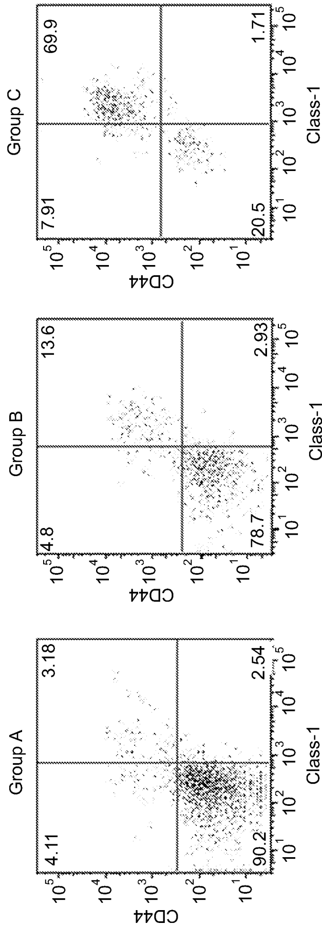
Comparison of Class-I and CD44 Expression in Groups A, B, and C
