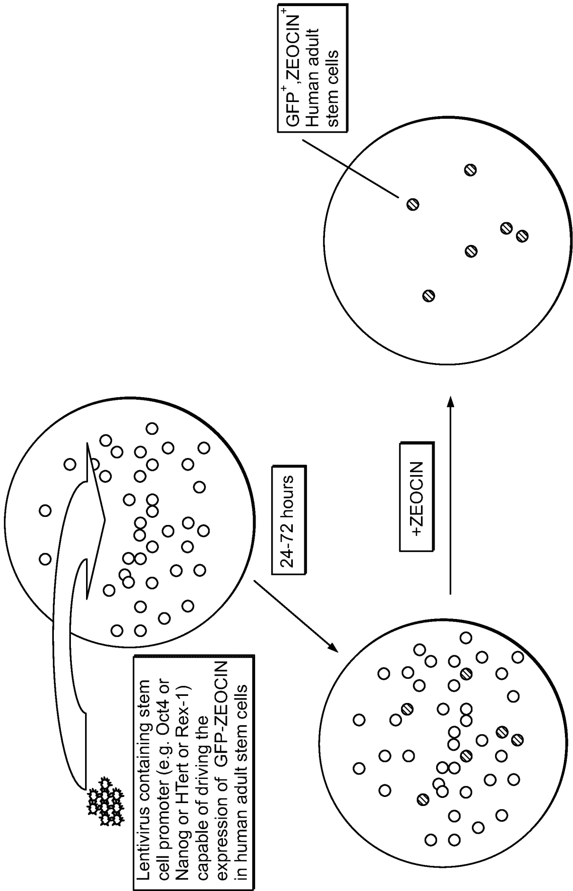
FIG. 10B Lentiviral transduction and ZEOCIN selection of human adult stem cells
