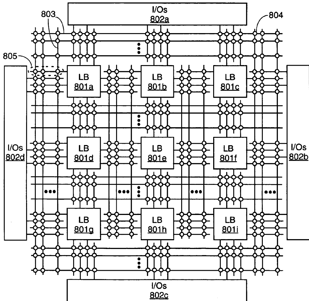
FIG. 8 (Prior Art)
