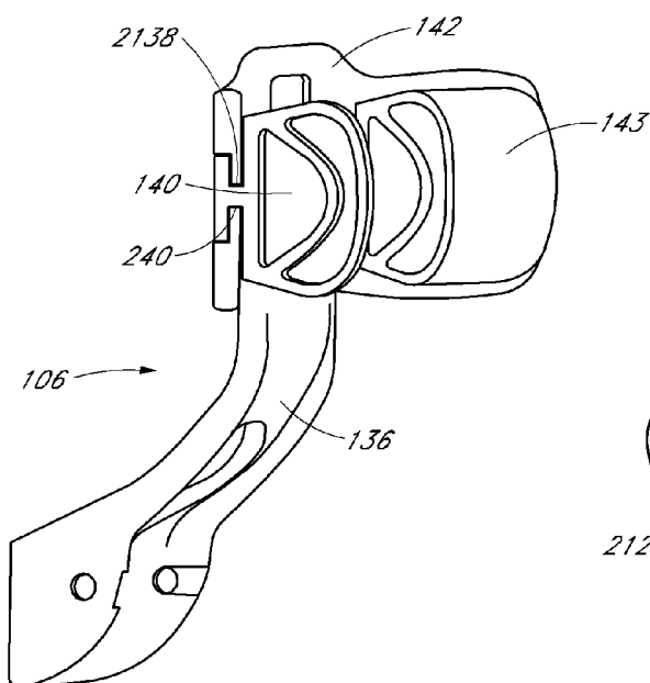
FIG. 7 (PRIOR ART)
