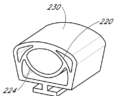
FIG. 11 (PRIOR ART)
