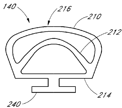
FIG. 8 (PRIOR ART)
