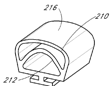
FIG. 9 (PRIOR ART)
