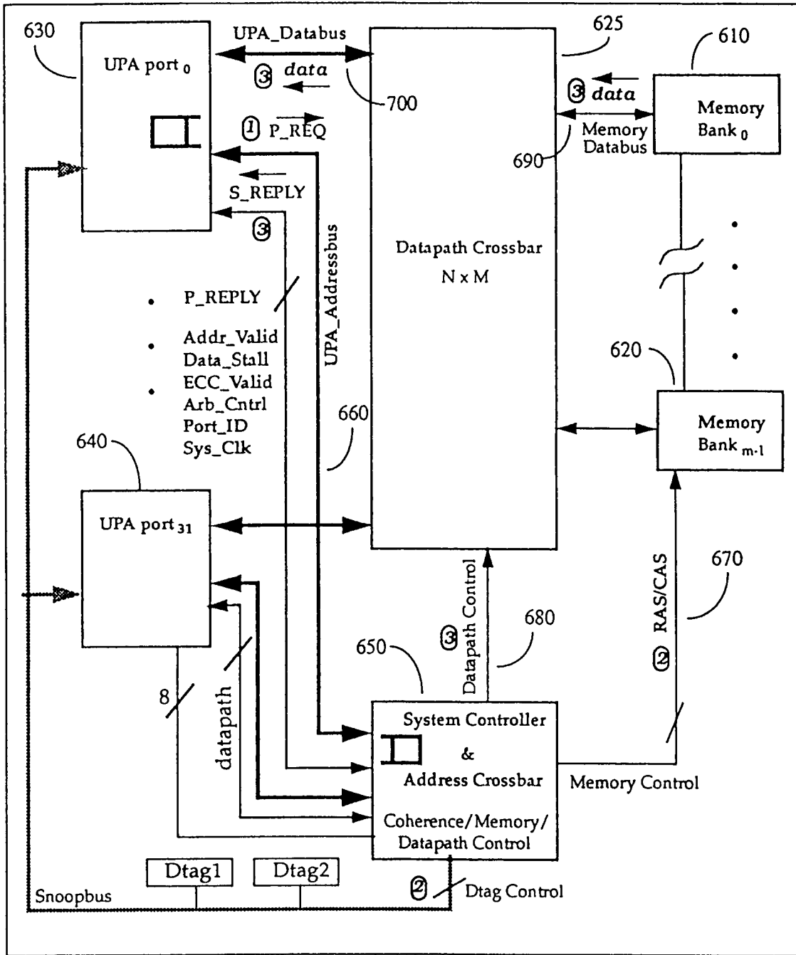
Memory Read Flow Control
