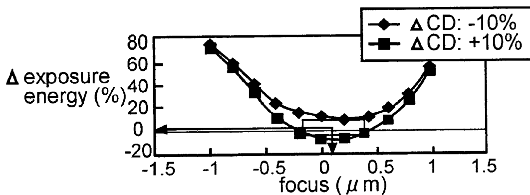
(1) without aberration
