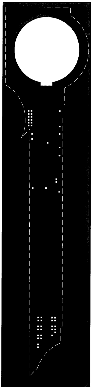
Via 1 mask
