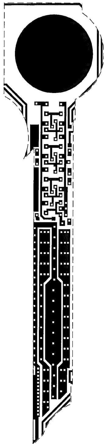
Metal 1 mask
