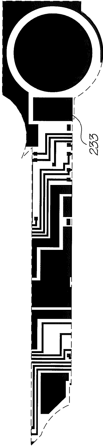
Metal 2 mask
