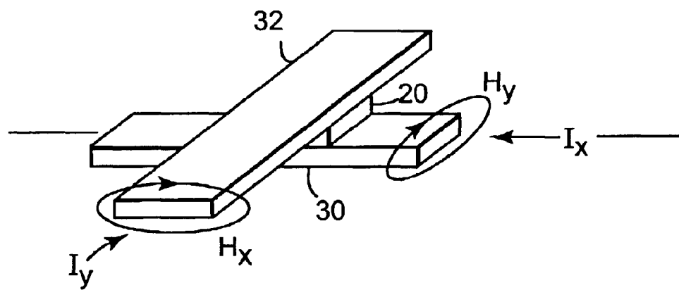
Fig. 2 (PRIOR ART)
